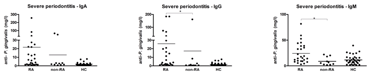
Figure 3 IgA, IgG, and IgM antibody response against Porphyromonas gingivalis in rheumatoid arthritis (RA) patients and non-RA controls with severe periodontitis as well as in healthy controls (HC). * P < 0.05 . Ig, immunoglobulin.
