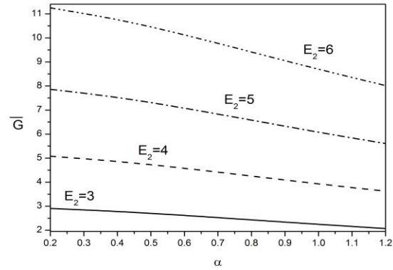
Fig. 7 : Effect of E_2 on \bar{G} (\varepsilon = 0.2, \beta = 5, E_1 = 0.1, E_3 = 0.06, M = 10, \mu_1 = 0.04)
