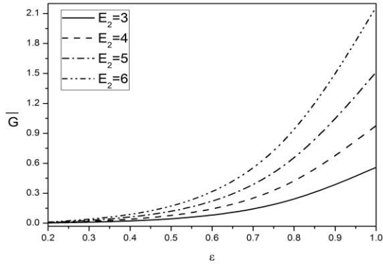
Fig. 6 : Effect of E_2 on \bar{G} (\beta = 5, \alpha = 0.5, E_1 = 0.1, E_3 = 0.06 M = 10, \mu_1 = 0.04)
