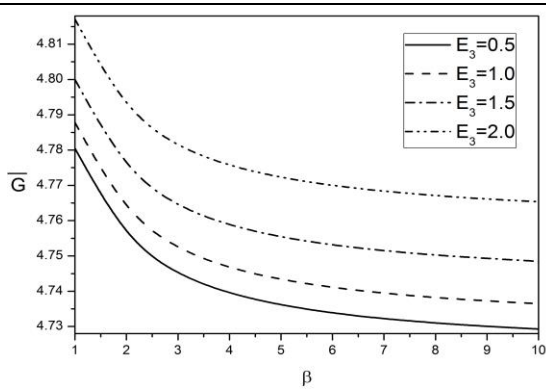
Fig. 8 : Effect of E_3 on \bar{G} (\varepsilon = 0.2, \alpha = 0.5, E_1 = 0.1, E_2 = 4.0, M = 10, \mu_1 = 0.04)
