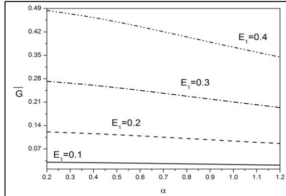
Fig. 4 : Effect of E_1 on \bar{G} (\varepsilon = 0.2, \beta = 5, E_2 = 0.0, E_3 = 0.06, \mu_1 = 0.04, M = 10)
