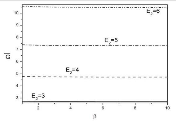
Fig. 5 : Effect of E_2 on \bar{G} (\varepsilon = 0.2, \alpha = 0.5, E_1 = 0.1, E_3 = 0.0, \mu_1 = 0.04, M = 10)
