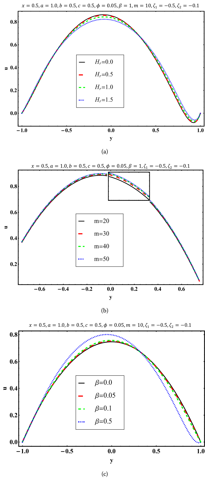
Figure 2 Variation of axial velocity u vs: (a) H_r , (b) m , (c) \beta , (d) \zeta_1 , and (e) \zeta_2 .
