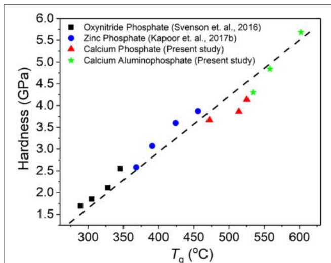
FIGURE 9 | Relationship between Vickers hardness ( H_V ) and T_g for various phosphate-based glasses (Svenson et al., 2016; Kapoor et al., 2017b). All the H_V values in the figure are obtained from tests conducted at 0.05 kgf load.
