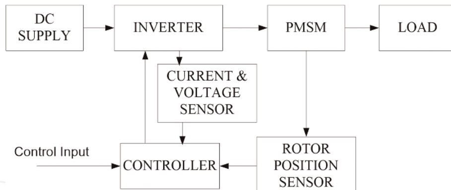
Figure 7. Components permanent magnet synchronous motor drive.
