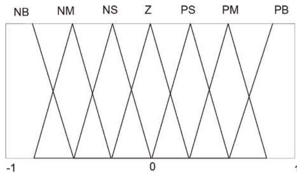
Figure 14. Change in torque error input to FLC.
