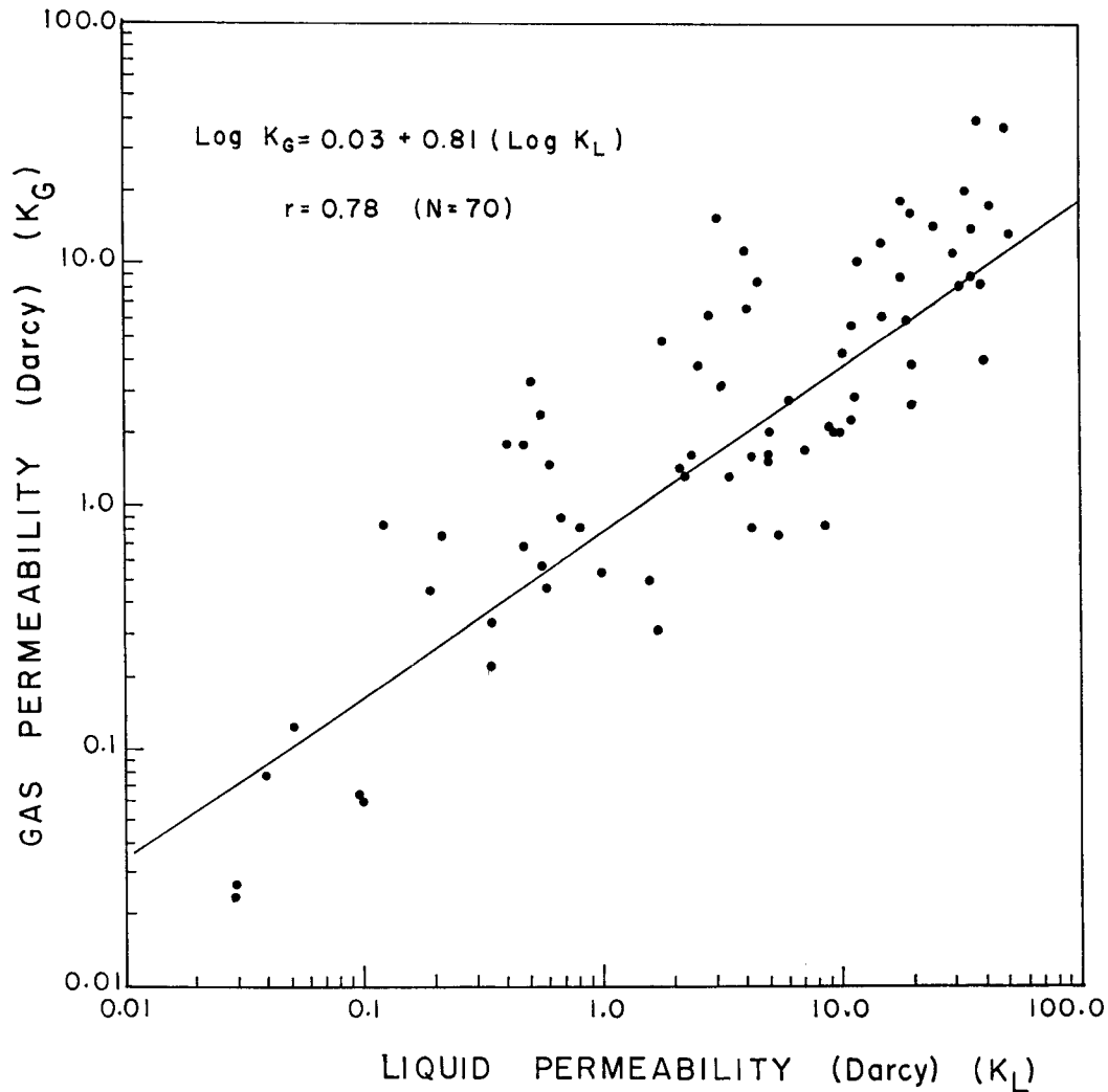
FIG. 4. Correlation between superficial gas permeability at 0% moisture content and liquid permeability.
