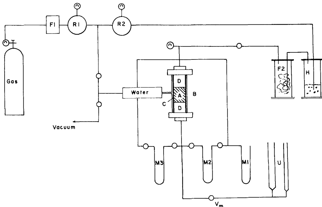
FIG. 1. Flow diagram of gas permeability apparatus. (A) wood sample, (B) permeability sample holder, (C) rubber sleeve, (D) steel plunger, (R1) 0-100 psig range pressure regulator, (R2) 0-30 psig range pressure regulator, (F1) gas filter, (F2) spun glass filter, (H) humidifier, (M1) mercury manometer for upstream pressure, (M2) mercury manometer for pressure drop, (M3) water manometer for pressure drop, ( V_m ) metering valve, and (U) bubble meters for measuring flow rates.
