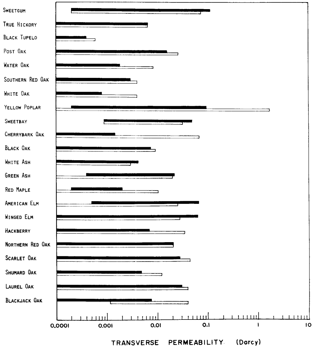
FIG. 3. Ranges of permeability values in the transverse directions for various hardwood species at 0% moisture content. Shaded bars are tangential movement; unshaded bars are radial movement.
