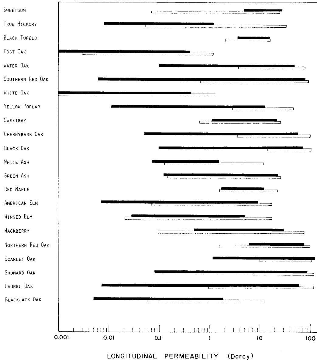
FIG. 2. Ranges of permeability values in the longitudinal direction for various hardwood species at 0% moisture content. Shaded bars are corewood; unshaded bars are sapwood.
