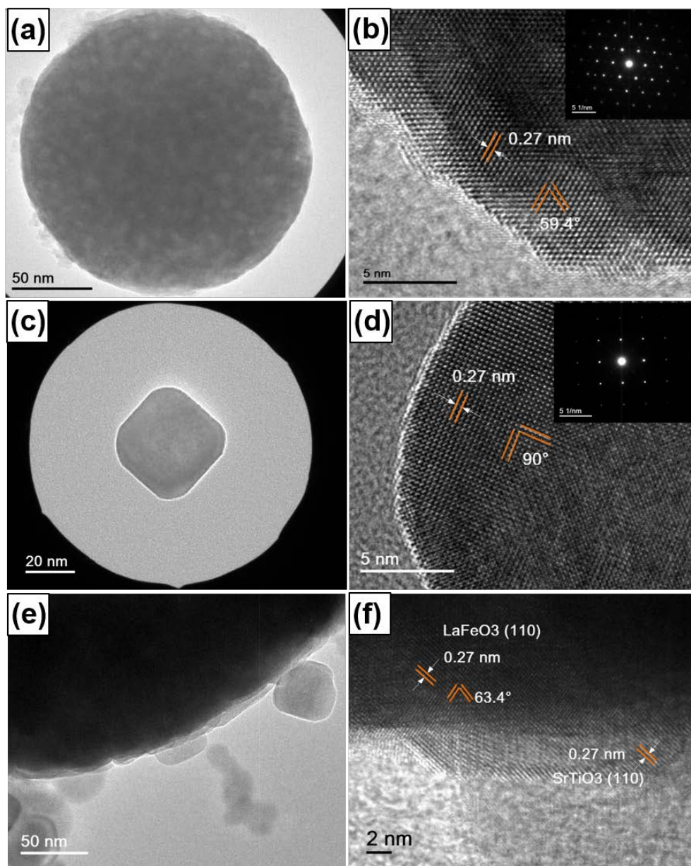
Figure 3. (a, b) Representative TEM and HR-TEM images of the as-prepared pristine LaFeO 3 with SAED patterns; (c, d) Representative TEM and HR-TEM images of the as-prepared pristine SrTiO 3 with SAED patterns; (e, f) Representative TEM and HR-TEM images of the as-prepared LFO-STO 0.3 composite interface.
