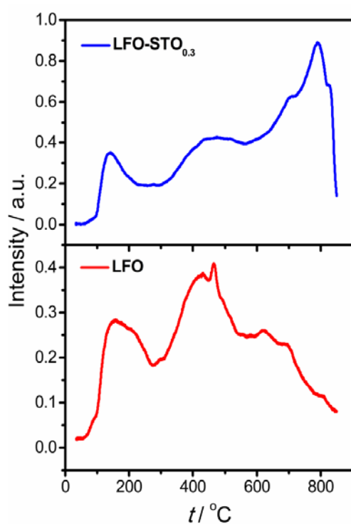
Figure 7. TPD profiles of NO for the as-prepared pristine LaFeO 3 and LFO-STO 0.3 composite
