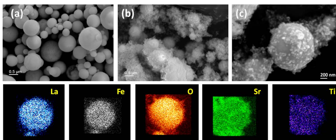
Figure 2. (a) Representative SEM images of the as-prepared LFO microspheres; (b, c) Representative SEM images of the as-prepared LFO-STO 0.3 composite at low and high magnifications; and EDX mapping images corresponding to (c).
