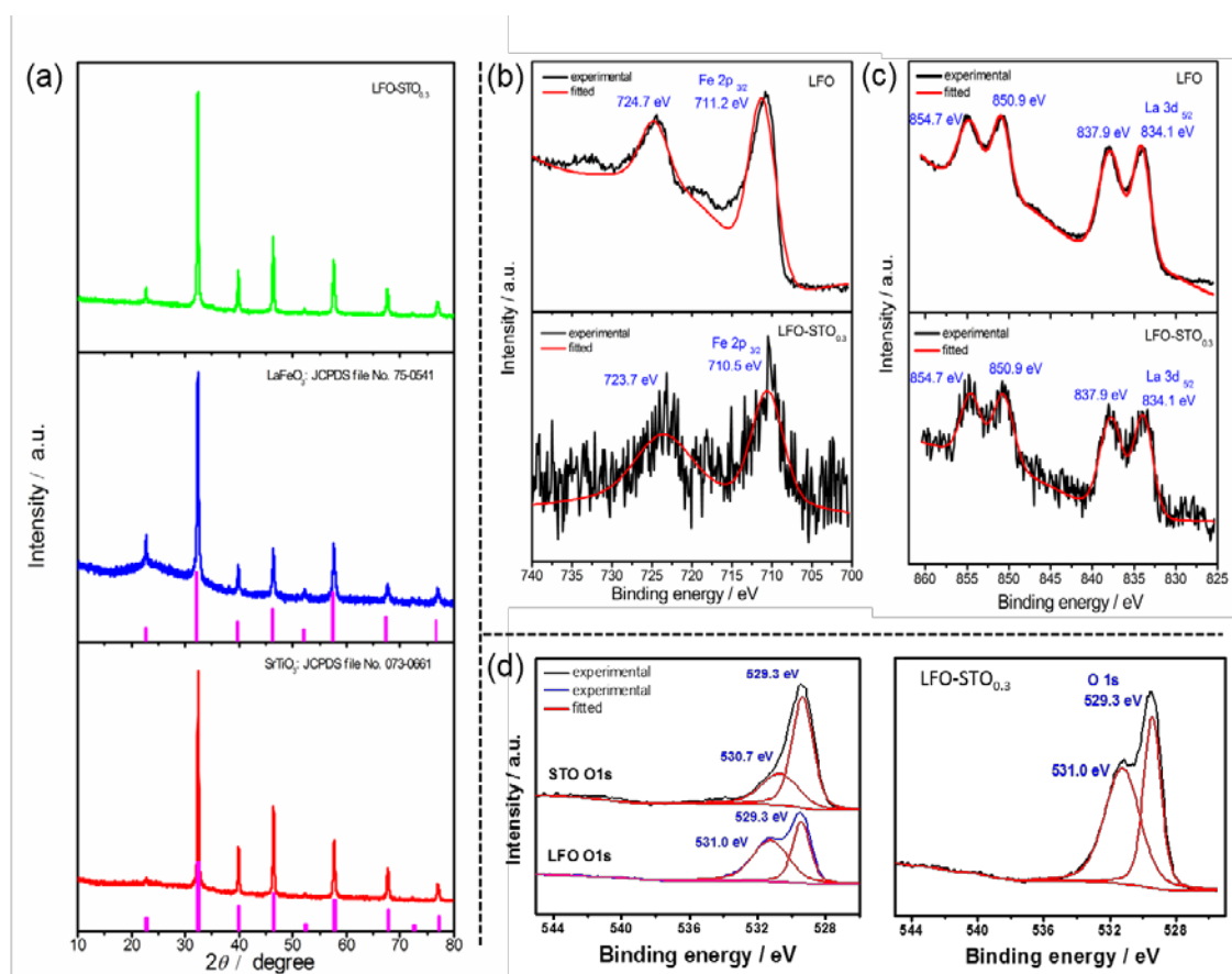
Figure 1. (a) Powder XRD patterns of the as-prepared pristine STO, LFO and LFO-STO 0.3 composite photocatalysts; (b) High resolution Fe 2p orbital XPS spectra of the LFO-STO 0.3 composite and LFO; (c) La 3d orbital spectra of the LFO-STO 0.3 composite and LFO; (d) O 1s orbital spectra of the pristine STO, LFO and LFO-STO 0.3 composite.
