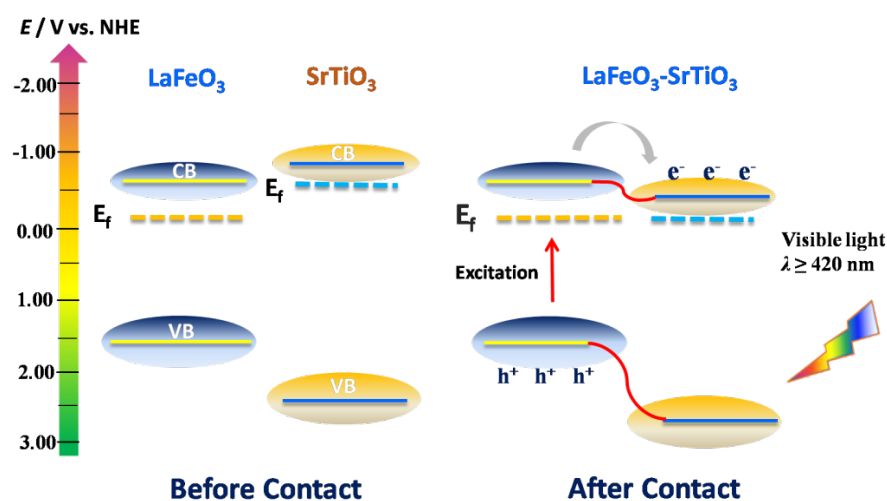
Scheme 1. Schematic band alignment and mechanism of charge transfer at the interface of the LaFeO 3 -SrTiO 3 composite under visible light irradiation ( \lambda \geq 420 nm)
