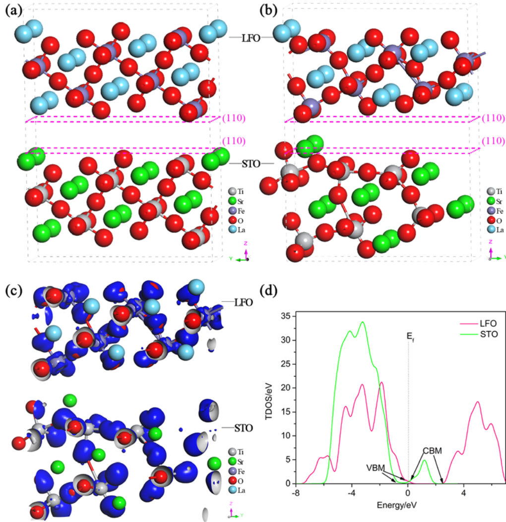
Figure 6. The crystal models (a) before and (b) after geometry optimization, (c) the calculated electron density difference (EDD) diagram (notice: blue area represents the increase of electron density) and (d) total density of states (TDOS) of the LFO-STO composite.
