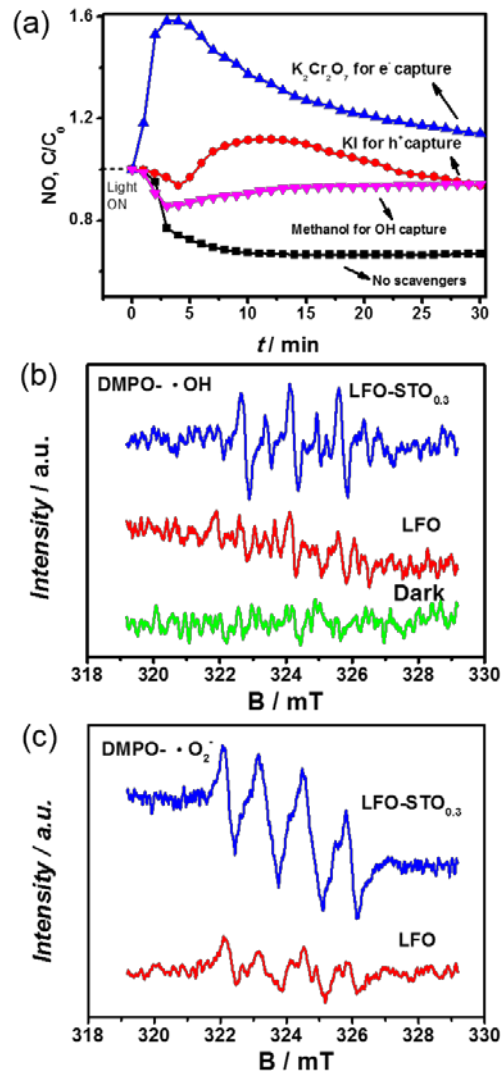
Figure 8. (a) NO removal profile under visible light irradiation with the addition of potassium dichromate, potassiumiodideand methanol as electrons, holes and •OH scavengers, respectively; (b) ESR signals of DMPO- •OH spin adduct in ethanol dispersion of the pristine LFO and LFO-STO 0.3 composite in the dark and under illumination for 3 minutes ( \lambda \geq 420 nm); (c) DMPO- •O 2 - spin adduct in ethanol dispersion of the pristine LFO and LFO-STO 0.3 composite under illumination for 3 minutes ( \lambda \geq 420 nm)
