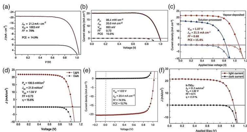
Fig. 9 J–V curves of various OMH perovskite devices: (a) \text{TiO}_2/\text{CH}_3\text{NH}_3\text{PbI}_3/\text{spiro-OMeTAD} , (b) \text{TiO}_2/\text{CH}_3\text{NH}_3\text{PbI}_3/\text{spiro-OMeTAD} , (c) \text{TiO}_2/\text{CH}_3\text{NH}_3\text{PbI}_{3-x}\text{Cl}_x/\text{spiro-OMeTAD} , (d) graphene- \text{TiO}_2/\text{meso-Al}_2\text{O}_3/\text{CH}_3\text{NH}_3\text{PbI}_{3-x}\text{Cl}_x/\text{spiro-OMeTAD} , (e) \text{ZnO}/\text{CH}_3\text{NH}_3\text{PbI}_3/\text{spiro-OMeTAD} , (f) \text{TiO}_2/\text{CH}_3\text{NH}_3\text{PbI}_{3-x}\text{Cl}_x/\text{spiro-OMeTAD} . Reproduced with permission from Ref. 20.
