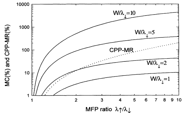
FIG. 3. Transmission characteristics of the spin-dependent transport. The relative change in magnetocurrent MC (%) and the relative change in perpendicular hot-electron spin valve effect in the base CPP-MR (%) are plotted versus the MFP ratio \lambda_{\uparrow}/\lambda_{\downarrow} .
