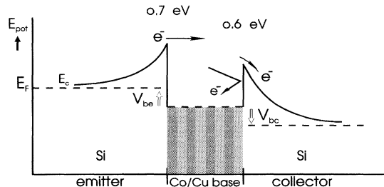
FIG. 2. Schematic energy band diagram of the spin-valve transistor under forward bias. The emitter Schottky barrier is slightly larger than the collector Schottky barrier, reducing quantum mechanical reflections. The collected electron current is exponentially dependent on the (inverse of the) MFP of the injected electrons in the Co/Cu multilayer base.
