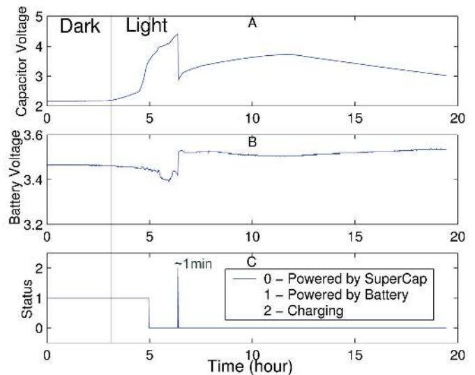
Fig. 10. Telos charges lithium battery from supercapacitors
