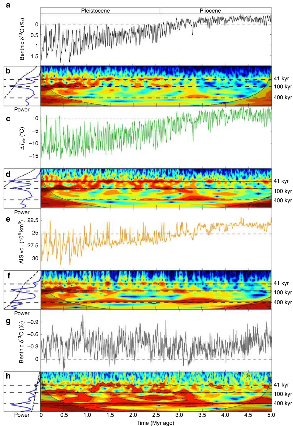
Figure 1 | Simulated variables and proxies with frequency wavelets. (a) Forcing record of the inverse routine, the LRO4 benthic \delta^{18}\text{O} stacked record 16 . (b) Wavelet analysis 48 of LRO4. (c) Simulated surface-air temperature anomaly ( ^{\circ}\text{C} ) over Antarctica and (d) wavelet analysis of temperature. (e) Simulated Antarctic ice volume ( 10^6 \text{ km}^3 ) and (f) wavelet analysis of ice volume. (g) Eastern equatorial Pacific Leg 138 benthic \delta^{13}\text{C} record 13 and (h) wavelet analysis of \delta^{13}\text{C} . For b,d,f,h , the >95\% confidence levels are indicated by the black lines, and horizontal dashed lines indicate the 41, 100 and 400 kyr frequencies. The light shading indicates possible distorted results due to edge effects of the time series. On the left, the total power spectrum with the 95% confidence level indicated by the dashed line.
