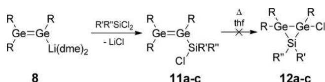
Scheme 6. Synthesis of \alpha -chlorosilyldigermenes 11 a–c ( \text{R} = \text{Tip} = 2,4,6\text{-}i\text{Pr}_3\text{C}_6\text{H}_2 ; 11 a , 12 a : \text{R}' = \text{R}'' = \text{Me} ; 11 b , 12 b : \text{R}' = \text{Me} , \text{R}'' = \text{Ph} ; 11 c , 12 c : \text{R}' = \text{R}'' = \text{Ph} ).
