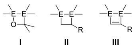
Scheme 1. Small ring systems (E = Si, Ge) derived from [2+2] cycloadditions of disilenes or digermenes to ketones (I), alkenes (II), and acetylenes (III).
