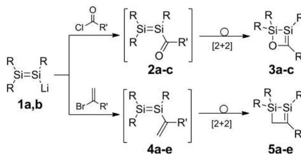
Scheme 2. Synthesis of cyclic silenes 3 a–c and 5 a–e ( 1 a : R = Tip = 2,4,6- i Pr 3 C 6 H 2 ; 1 b : R = SiMe 2 Bu 2 ; 2 a , 3 a : R = Tip, R' = t Bu; 2 b , 3 b : R = Tip, R' = 1-adamantyl; 2 c , 3 c : R = SiMe 2 Bu 2 , R' = 1-adamantyl; 4 a , 5 a : R = Tip, R' = Ph; 4 b , 5 b : R = Tip, R' = SiMe 3 ; 4 c , 5 c : R = SiMe 2 Bu 2 , R' = H; 4 d , 5 d : R = SiMe 2 Bu 2 , R' = Ph; 4 e , 5 e : R = SiMe 2 Bu 2 , R' = SiMe 3 ). [8,9]
