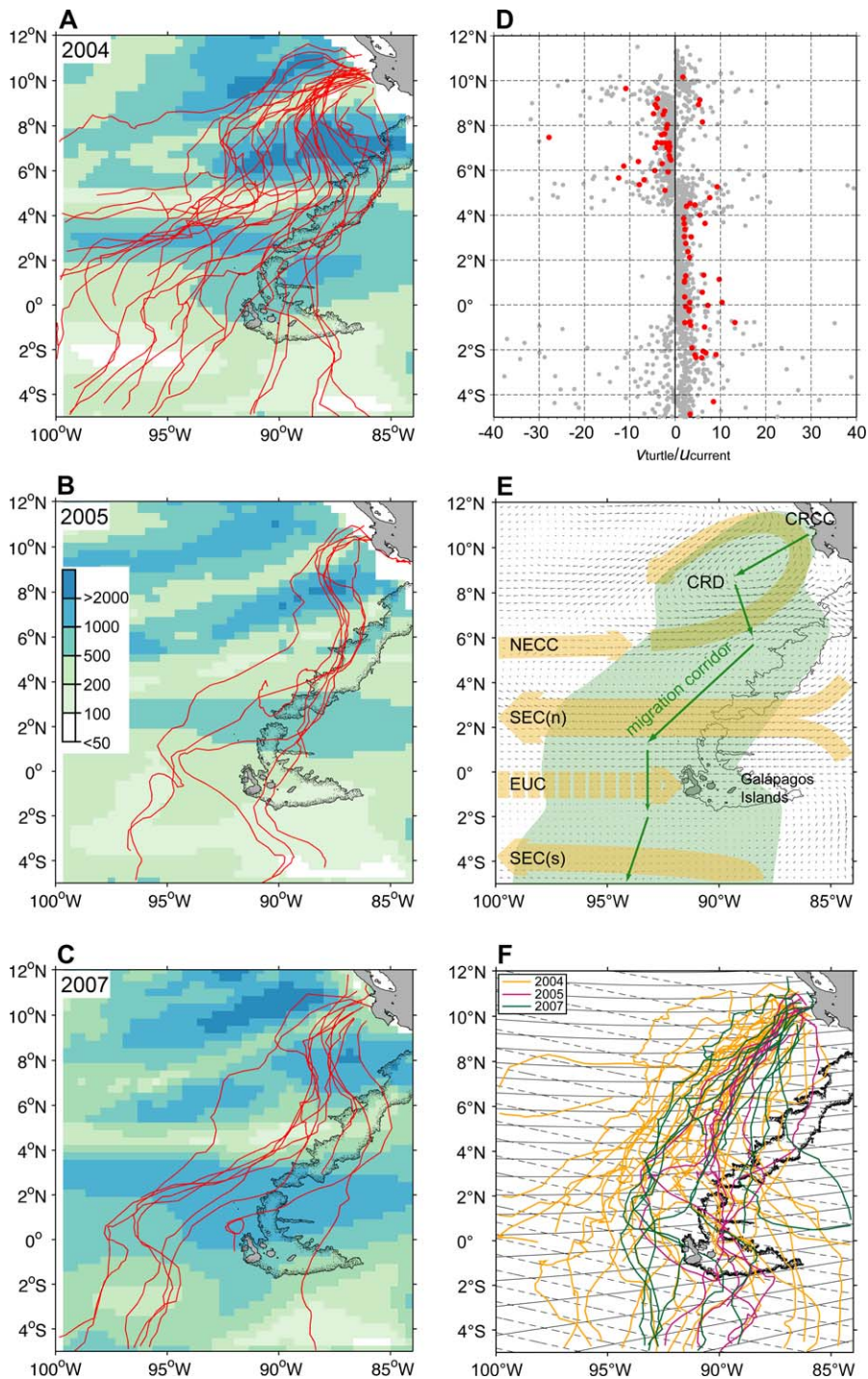
Figure 3. Leatherback Movements in Relation to Ocean Currents in the Migration Corridor Region
