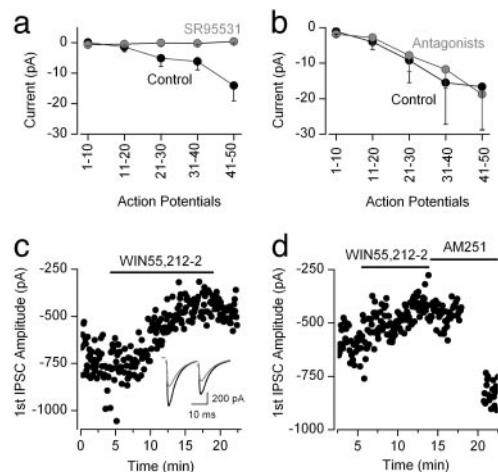
Fig. 5. Pharmacological properties of unitary and evoked IPSCs. (a) The selective GABA A receptor antagonist SR95531 (>20 \mu M) abolished the PSCs evoked by presynaptic AP trains in MFA INs ( n = 3 ). (b) A mixture of receptor antagonists (50 \mu M LY341495, a broad-spectrum mGluR; 10 \mu M CGP55845, a GABA B ; and 1 \mu M atropine, a muscarinic antagonist) did not affect IPSCs evoked by high-frequency trains of APs (50 APs at 100 Hz) in MFA INs ( n = 4 ). (c) A CB 1 receptor agonist (1 \mu M WIN55,212-2) reduces the amplitude of the extracellular-stimulation-evoked IPSCs by 39% in a CA1 PC. (Inset) Averaged traces in control (black trace) and in WIN55,212-2 (gray trace). (d) Compound IPSCs evoked in CA3 PCs were reduced (28%) by the CB 1 receptor agonist (1 \mu M WIN55,212-2). Consecutive application of the CB 1 antagonist (10 \mu M AM251) not only reversed the effect of the agonist but also resulted in an additional 49% increase in IPSC amplitudes. The stimulation had to be stopped for 4 min during the antagonist wash-in period for technical reasons.
