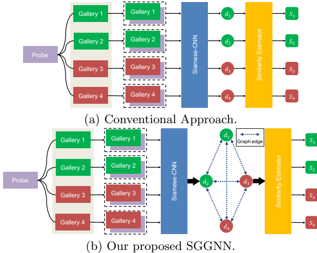
Fig. 1. Illustration of our Proposed SGNN method and conventional person re-identification approach. (a) The pipeline of conventional person re-identification approach, the pairwise relationships between different probe-gallery pairs are ignored. The similarity score of each probe-gallery pair d_i ( i = 1, 2, 3, 4 ) is estimated individually. (b) Our proposed SGNN approach, pairwise relationships between different probe-gallery pairs are involved with deeply learned message passing on a graph for more accurate similarity estimation.
