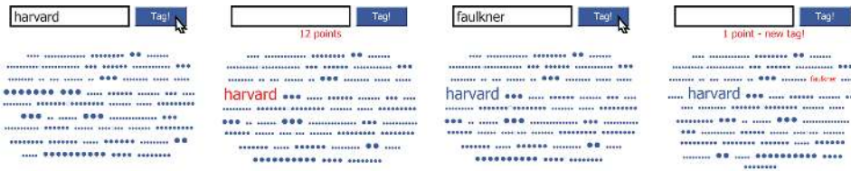
Fig. 2. The tag cloud begins completely obscured. The player guesses harvard , receives 12 points for agreeing with eleven other players and reveals Harvard as a large tag. Faulkner is next; it does not match existing tags and is added to the cloud.
