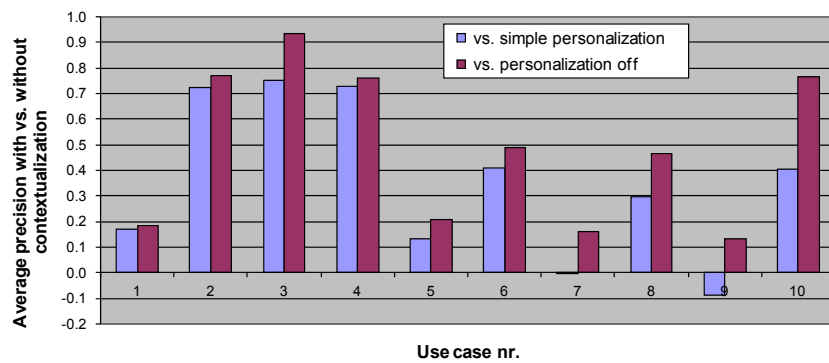
Figure 7 Comparative precision histogram of personalized search with and without contextualization for the ten use cases. The light-colored bars compare personalized retrieval in context vs. simple personalized retrieval without context, and the dark-colored ones compare personalized retrieval in context vs. retrieval without personalization.
