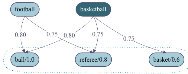
Figure 2 Fuzzy taxonomic context example.
