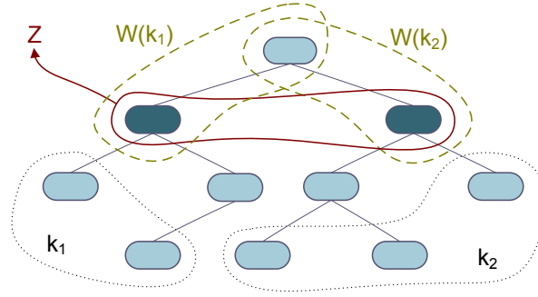
Figure 3 Relation T and fuzzy preferences extraction example.
