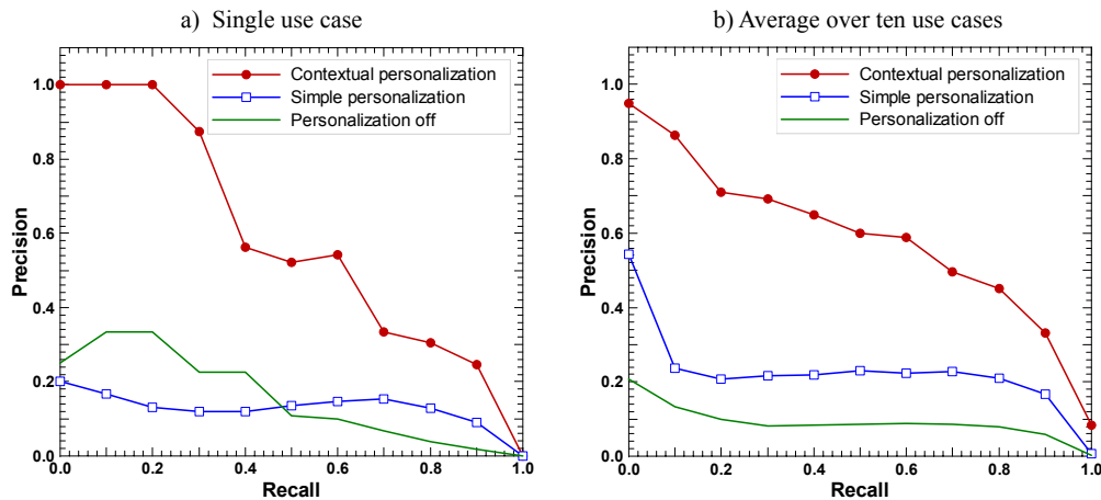
Figure 6 Comparative performance of personalized search with and without contextualization, showing the precision vs. recall curve for a) one of the scenarios, and b) the average over 10 scenarios. The results in graphic a) correspond to the query “Companies based in any Japanese region”, from the use case described in Section 6.
