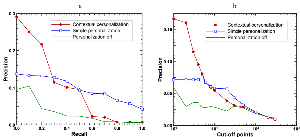
Figure 8 Comparative performance of personalized search with and without contextualization tested with 18 subjects on three proposed tasks. The graphics show a) the precision vs. recall curve, and b) the precision at cut-off points. The results are averaged over the set of all users and tasks.
