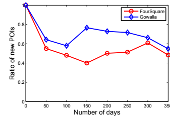
Figure 1: The ratio of new POIs with number of days on two real-world datasets.
