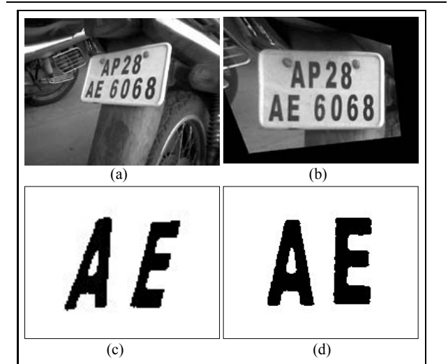
Figure 1. Original Image of a license plate (a) and its perspective corrected version (b). Two selected characters ('A' and 'E') are shown before (c) and after (d) rectification.
