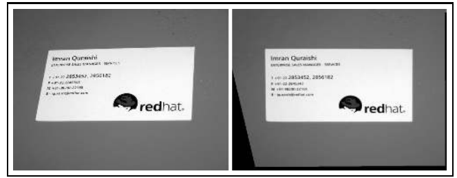
Figure 3. A perspective image of a visiting card is rectified with the help of its bounding rectangle.
