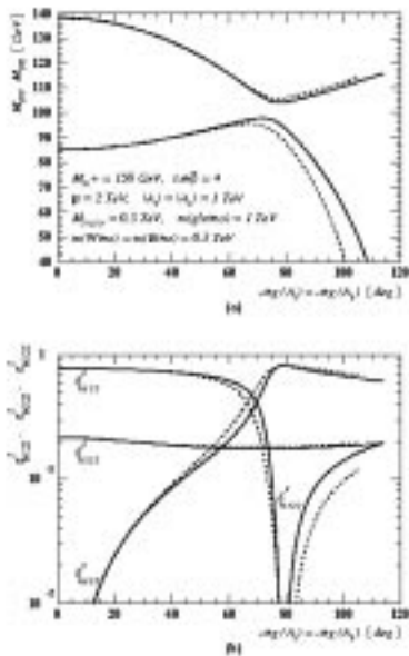
Figure 11: Illustration how CP violation in the MSSM may suppress the coupling of the lightest neutral Higgs boson to the Z [56].
