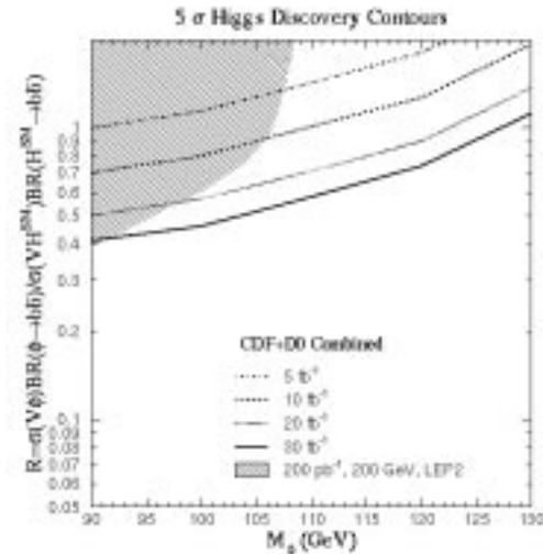
Figure 2: Higgs discovery sensitivity of the Fermilab Tevatron collider compared with that of LEP [10].
