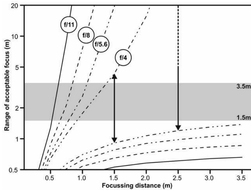
Figure 7. Focussing distance and corresponding range of acceptable focus with varying aperture, based on 8 mm focal length lens and 1/1.7" [7.44 x 5.58 mm] image sensor size, a common commercially-available deep-water camera system.
