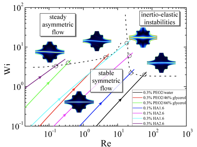
FIG. 5. A stability diagram for viscoelastic flow of dilute solutions of poly(ethylene oxide) (PEO) and hyaluronic acid (HA) through an OSCER (Optimized Shape Cross-slot Extensional Rheometer) device. The elasticity number of each fluid (shown by the colored lines of constant \text{Wi}/\text{Re} ) are varied by changing the polymer concentration or solvent viscosity. Two distinct modes of instability can be observed at high Weissenberg and Reynolds numbers [90].
