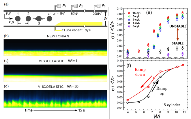
FIG. 8. Nonlinear elastic instability in a microfluidic channel flow. (a) Experimental setup showing the initial linear array of cylinders followed by a long parallel shear flow region. (b,c,d) Space-time dye patterns for the case with 15-cylinders for Newtonian and polymeric fluids measured far downstream. (e) Normalized velocity fluctuations as a function of initial perturbation ( n ) and Wi showing the appearance of two branches. (f) Hysteretic behavior, a hallmark of nonlinear sub-critical instabilities, found for polymeric fluids [26].
