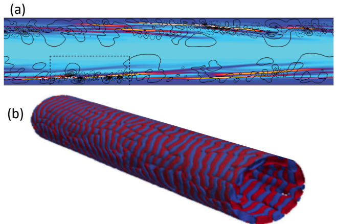
FIG. 18. Snapshots of simulations of EIT in (a) channel flow [300] and (b) pipe flow [299]. In (a) color contours indicate polymer stretching and lines indicate the magnitude Q of the second invariant of the velocity gradient tensor; reproduced with permission from [300]. In (b) isosurfaces indicate Q ; licensed under a Creative Commons Attribution (CC BY) license.
