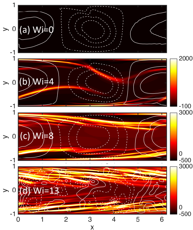
FIG. 20. Snapshots of the finite amplitude Tollmien-Schlichting wave solution at Re = 10000 and (a) Wi = 0 , (b) Wi = 4 , (c) Wi = 8 , (d) Wi = 13 [307]. White contours are wall-normal velocity and colors are deviations of xx polymer stretch from laminar values.
