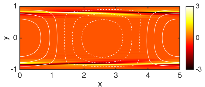
FIG. 19. Snapshot of the finite amplitude Tollmien-Schlichting wave solution at Re = 3000 , Wi = 10 [306]. White contours are wall-normal velocity, colors are deviations of xx polymer stretch from laminar values. Reproduced with permission from [306].
