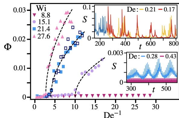
FIG. 7. Active control of elastic turbulence. Order parameter versus inverse Deborah number, De^{-1} , for different Wi ; here, De is defined as the product of the outer cylinder reversal frequency and the fluid stress relaxation time, while Wi is defined as the product of the outer cylinder maximum angular velocity and the fluid stress relaxation time. Insets: Secondary-flow strength versus time for different De at Wi = 21.4 . The time-modulated driving is switched on at t = 250 . Adapted from Ref. [162].
