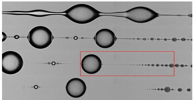
FIG. 25. The late stages of the blistering process of an aqueous 1000 ppm PEO solution [408]. The first image is at t = 250 ms after the formation of the cylindrical filament; subsequent images are taken every 30 ms. A thin fiber with the small beads is drawn out of the large droplet (red box). The width of the image is about 300 \mu\text{m} . Image is from R. Sattler, S. Gier, J. Eggers, and C. Wagner, Phys. Fluids 24 , 023101, (2012); licensed under a Creative Commons Attribution (CC BY) license.
