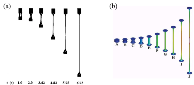
FIG. 24. Extensional necking. (a) Experiments of exponential elongation of a filament of a viscoelastic fluid (0.31 wt % polyisobutylene in polybutene) [357]. Reprinted from [Sridhar], with permission from Elsevier. (b) Numerical simulations of the so-called pom-pom model for an imposed strain rate \dot{\epsilon} , with the color scale indicative of the tensile stress [377]; see figure 9 of the reference for the time of each image. Reproduced from [377], with the permission of the Society of Rheology.
