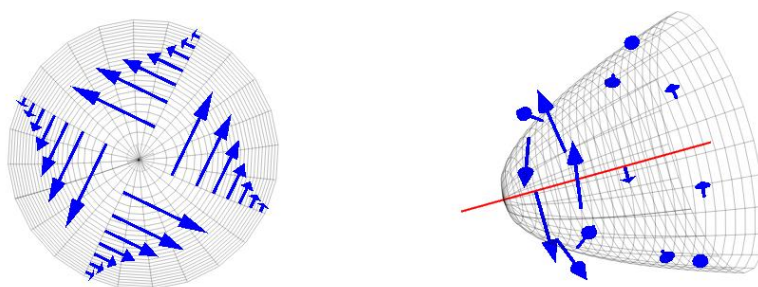
Figure 1. Left figure: top view of the cigar with the background gauge field schematically shown. Right figure: side view of the cigar and the background gauge field.
