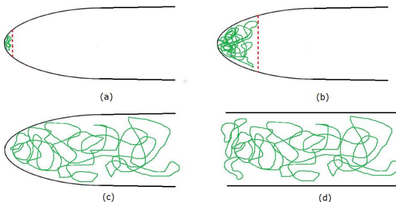
Figure 5. (a) Large k cigar background with random walk superimposed. Of course, in reality the random walk is on the spatial submanifold only, but for illustrative purposes we draw it like this. The (red) dashed line limits the spread of the discrete thermal scalar in the radial direction. For very large k the flat Rindler approximation becomes accurate. (b) Lowering k causes the discrete mode to spread radially. This invalidates the Rindler approximation. Nonetheless, the mode retains its dominant character. (c) When k = 1 , the mode spreads without bound radially. The mode becomes non-normalizable and disappears from the spectrum. Precisely at this point, the continuous thermal scalar takes over the dominant behavior. (d) The same dominant random walk on the linear dilaton background. The asymptotic parts of the random walks look the same for k = 1 .
