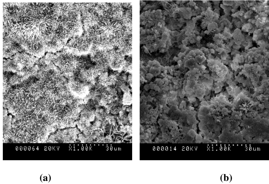
Figure 4.12: Hitachi SEM image of a) plain pervious concrete with no TiO 2 (PPC) and b) TiO 2 sprinkled on pervious concrete when it was fresh (SFC, sample WMS4) at 1000 times magnification
