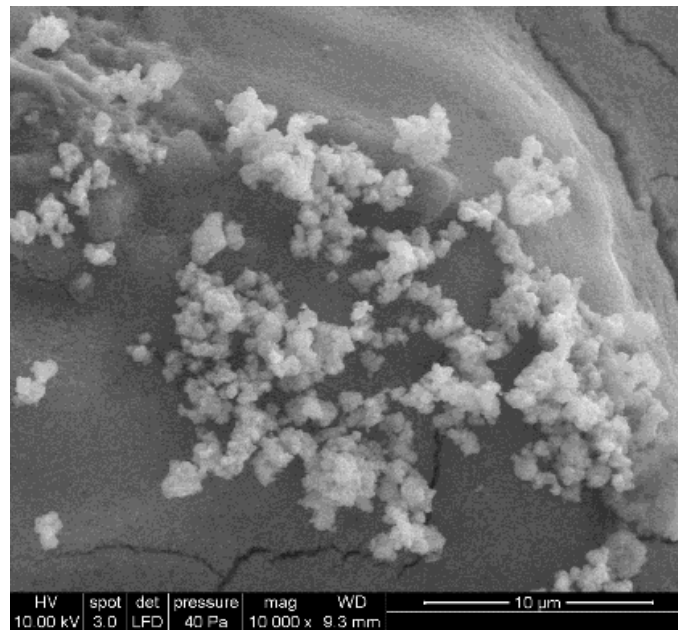
Figure 4.14: FEI SEM image of pervious concrete treated with commercial water-based TiO 2 (CWB) at 10,000 times magnification
