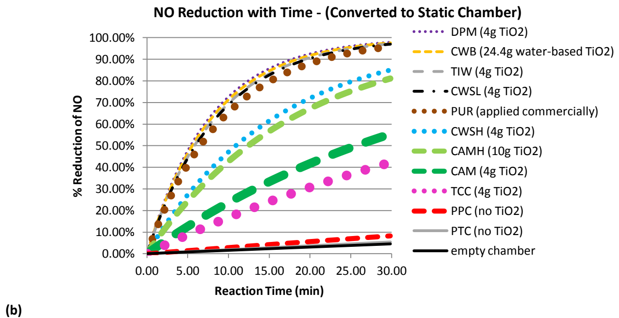
Figure 4.7: Results for NO reduction for final-evaluation samples with (a) flow-through chamber data and (b) converted to static chamber data
