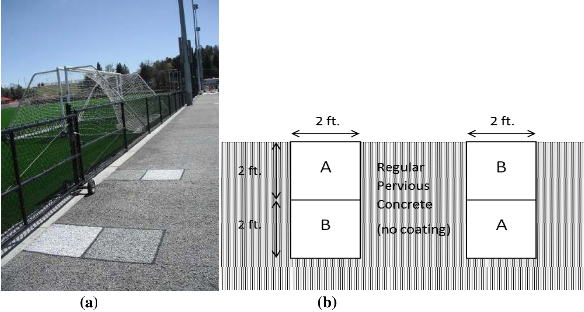
Figure 4.19: (a) Field coatings on the pervious concrete sidewalk a) on the first day of placement, and b) a diagram showing the placement of each coating, with coating A: driveway protector mix (DPM) and coating B: commercial water-based TiO 2 (CWB)
