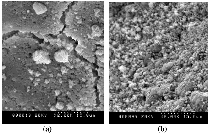
Figure 4.13: Hitachi SEM image of a) pervious concrete treated with cement-water slurry (CWSH, sample WMA9) and b) pervious concrete treated with driveway protector mix (DPM, sample WMC7) at 2000 times magnification
