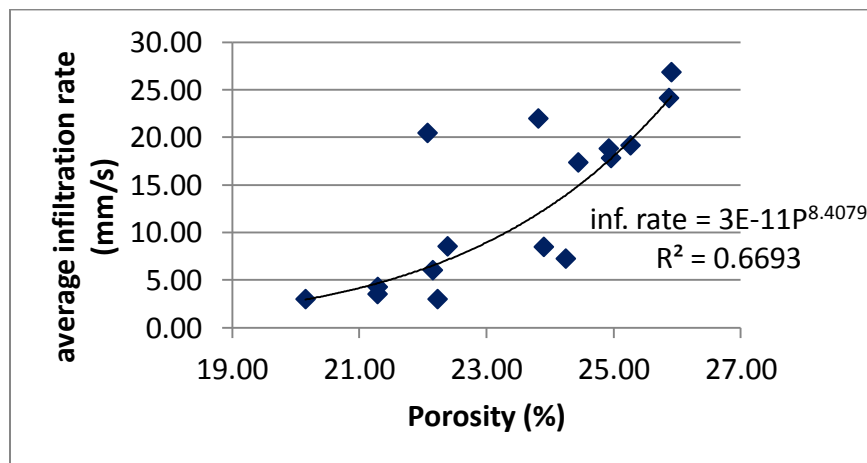
Figure 3.4: Infiltration rate vs. porosity for WMA and WMB samples
