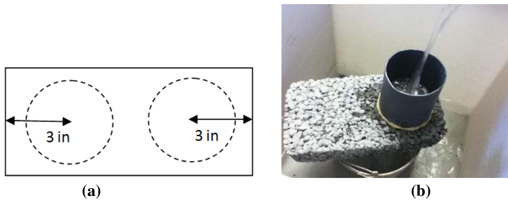
Figure 3.2: Water infiltrating completely through a pervious concrete sample
