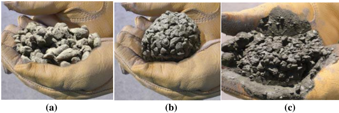
Figure A.3: The pervious concrete ball test when a) the ball crumbles (not enough water), b) the ball is good (just the right amount of water), and c) the ball loses its void structure (too much water) (“Pervious Concrete: Mix Design and Materials,” n.d.)
