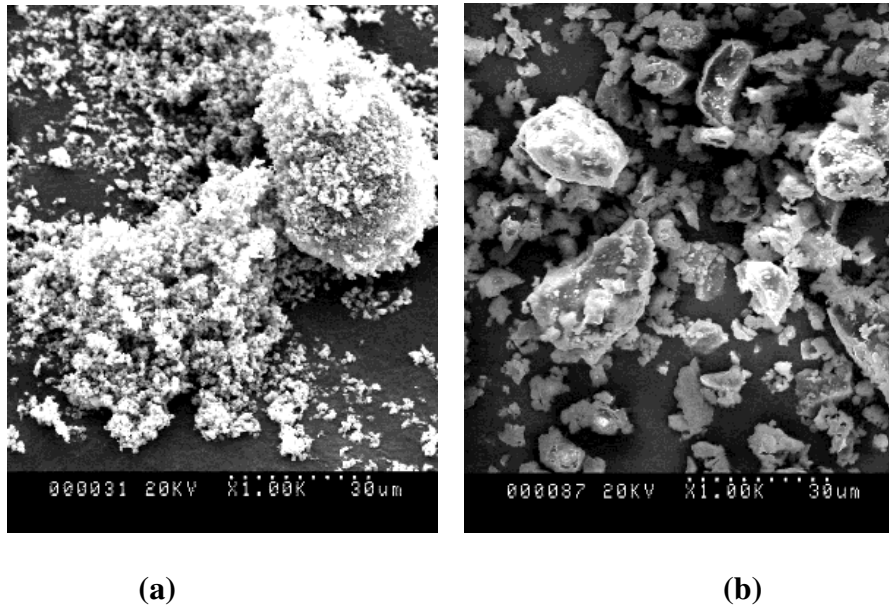
Figure 4.11: Hitachi SEM images of a) TiO 2 powder alone and b) cement powder alone at 1000 times magnification
