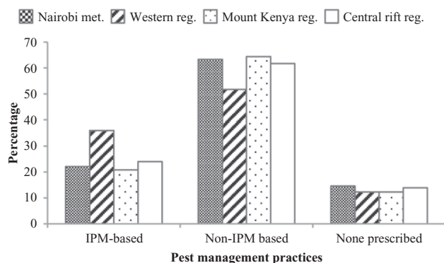
Fig. 5. Percentage distribution of intervention measures based on extension officers' location.
