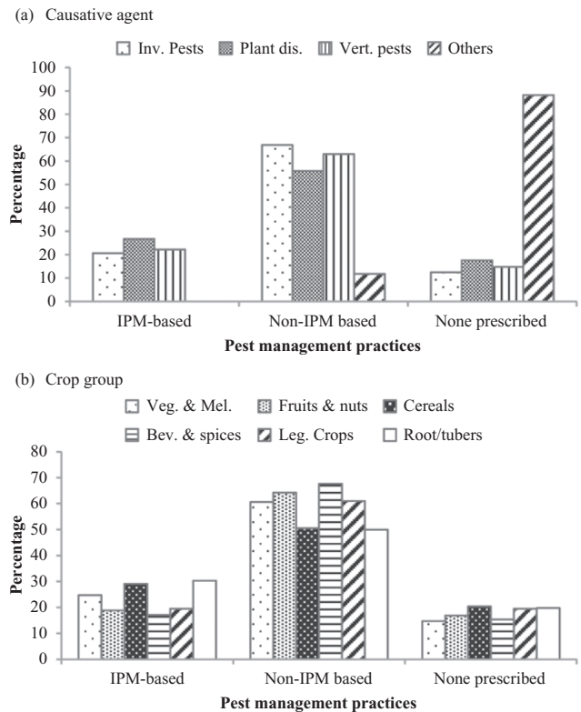
Fig. 6. Percentage distribution of intervention measures based on (a) causative agent, and (b) crop group.
