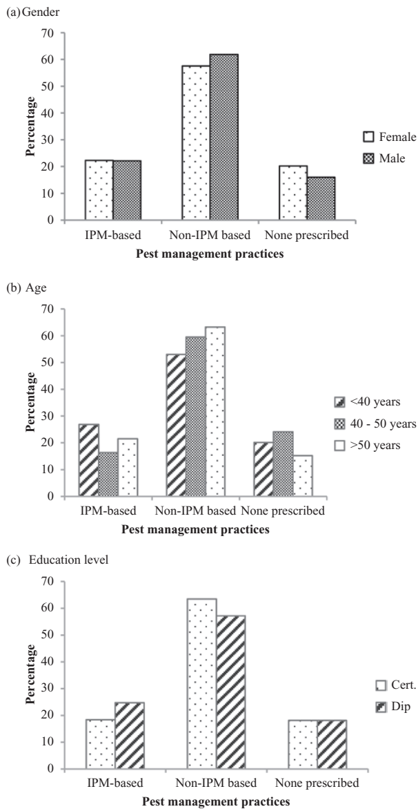
Fig. 4. Percentage distribution of intervention measures based on extension officers' (a) gender, (b) age, and (c) education level.
