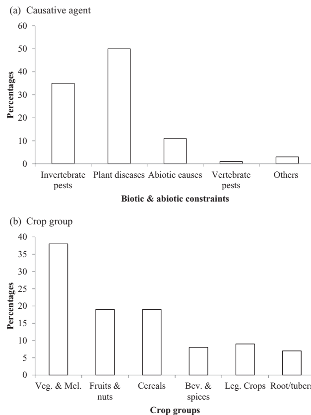
Fig. 1. Percentage distribution of (a) causative agent, and (b) crop group in the smallholder agricultural subsector of Kenya.
