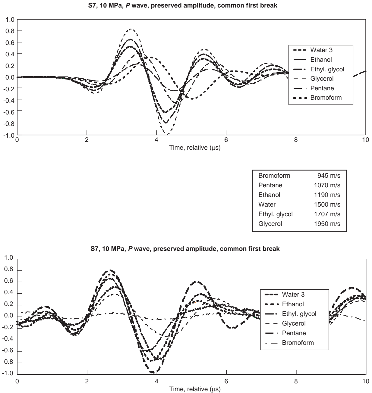
Figure 8 Estaillasses limestone: P and S waves propagated for various saturation states.
