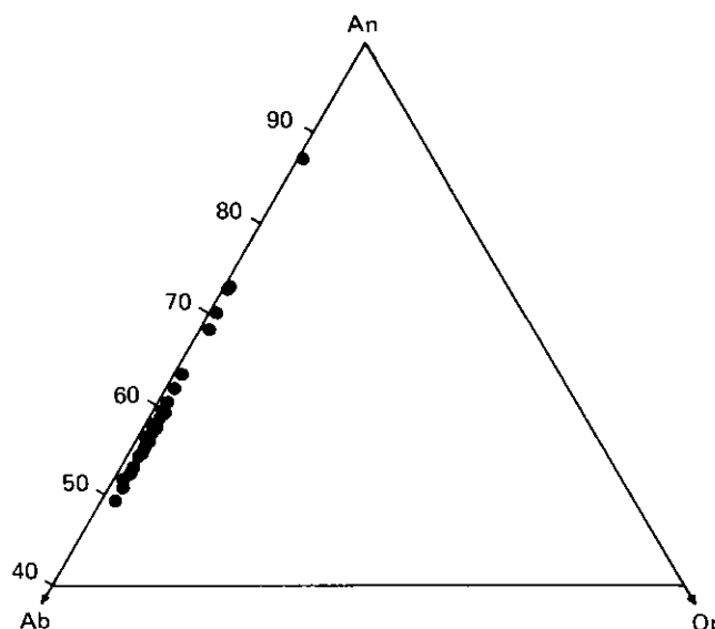
Figure 16. Part of albite(An)-anorthite(An)-orthoclase(Or) feldspar diagram showing compositions of cores of plagioclase grains from Yantarni volcanic rocks.
