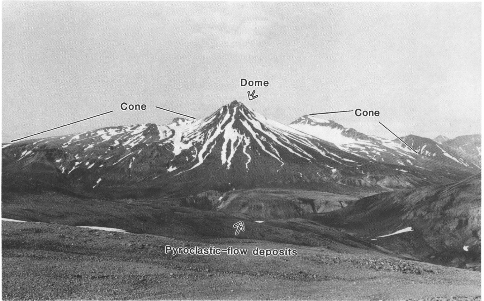
Central dome of Yantarni Volcano, 5 km distant, and flat-topped pyroclastic-flow deposits in middle foreground. View west.
