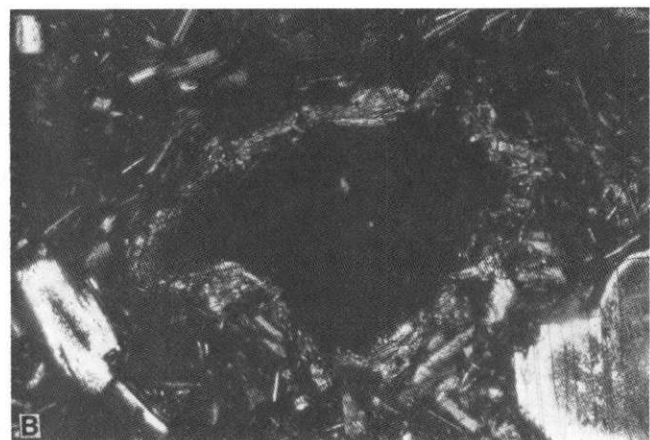
Figure 20. Photomicrographs of high-silica andesite composing Yantarni dome, showing quartz grain surrounded by a narrow reaction rim of clinopyroxene. Width of views, 1.5 mm; sample 39. A, Uncrossed polars. B, Crossed polars.
