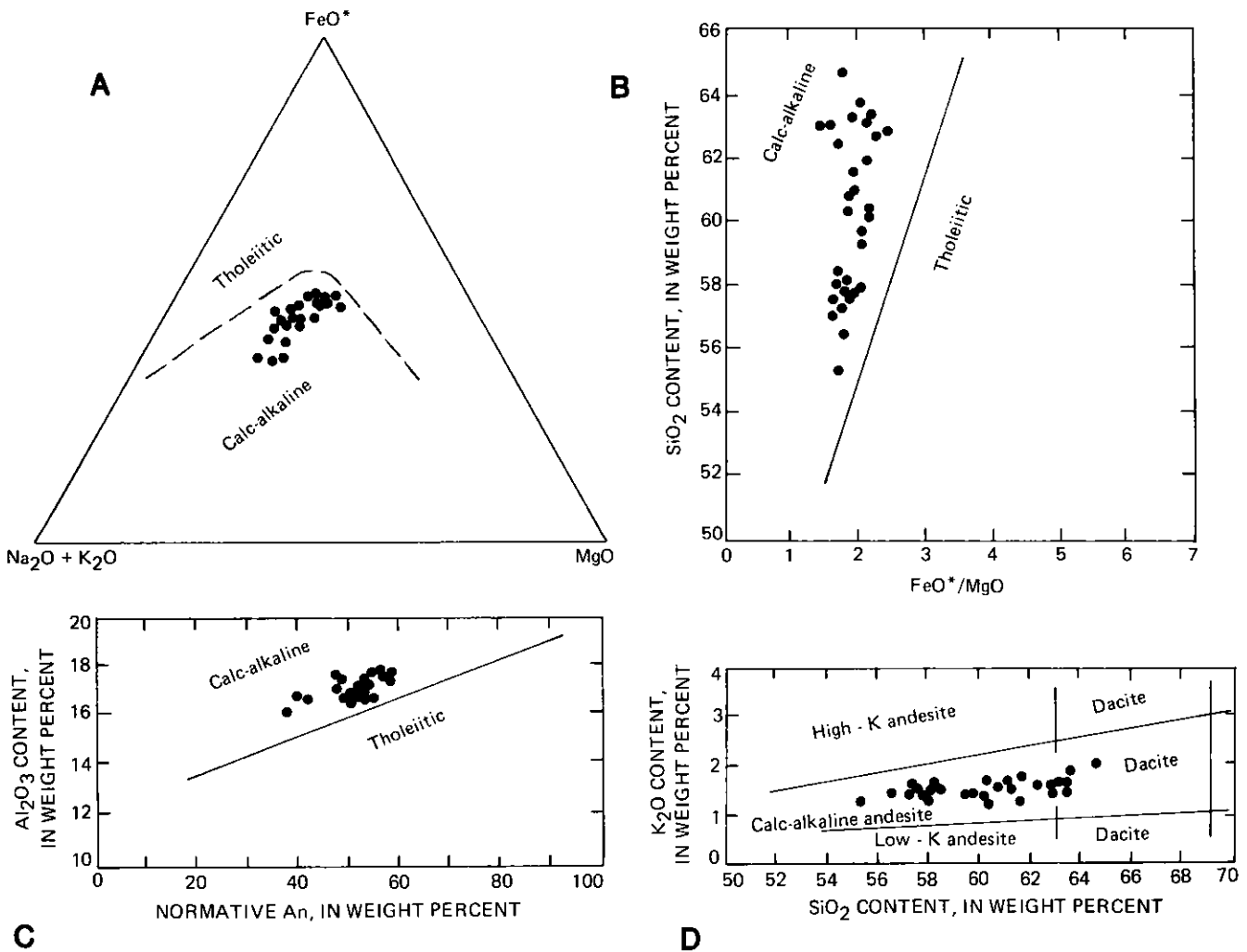
Figure 14. Classification plots of all Yantarni samples. A, FMA plot. Field boundary from Irvine and Baragar (1971). FeO^* = FeO + 0.9Fe_2O_3 . B, FeO^*/MgO versus SiO_2 . Field boundary from Miyashiro (1974). C, Al_2O_3 versus normative An. Field boundary from Irvine and Baragar (1971). D, K_2O-SiO_2 classification (Peccerillo and Taylor, 1976).
