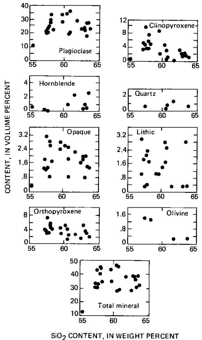
Figure 22. Phenocryst modes, lithic abundances, and total phenocryst contents plotted against whole-rock SiO_2 content (volatile-free) for Yantarni lavas. No plotted quantity shows any consistent correlation with SiO_2 .
