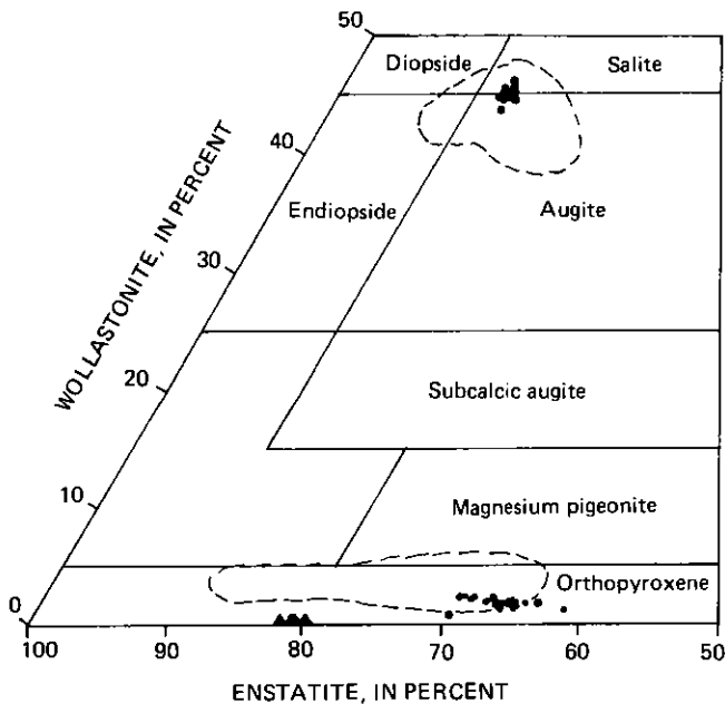
Figure 15. Pyroxene quadrilateral showing compositions of cores of clinopyroxene and orthopyroxene grains from lavas of Yantarni Volcano, relative to that of other medium-K calc-alkaline andesites (dashed lines; Gill, 1981). Olivine analyses (triangles) are projected onto baseline.
