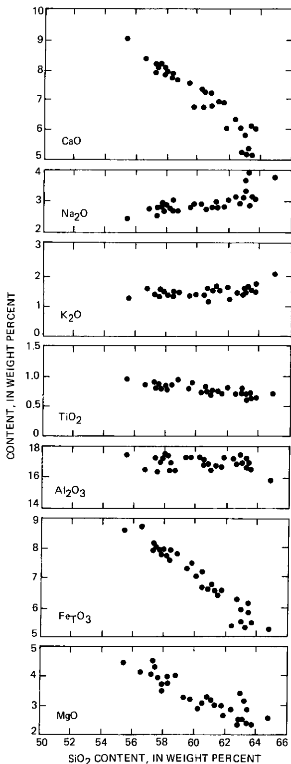
Figure 13. \text{SiO}_2 -variation diagrams of Yantarni volcanic rocks. Plotted values are normalized to 100 percent on a volatile-free basis but including \text{MnO} and \text{P}_2\text{O}_5 .
