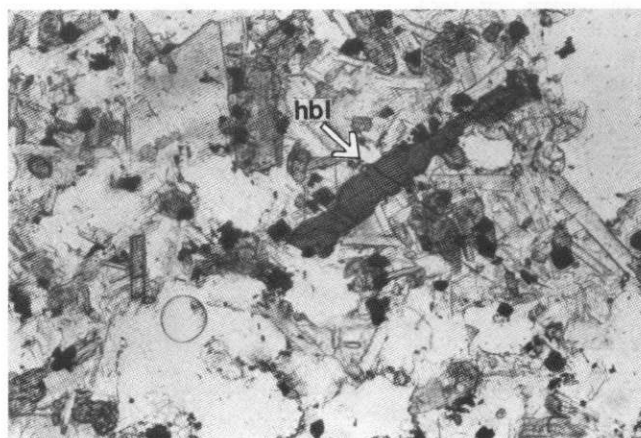
Figure 18. Photomicrograph of Yantarni basaltic andesite showing an unaltered hornblende microphenocryst (hbl) in fine-grained groundmass. Width of view, 1.5 mm. Uncrossed polars; sample 11b.
