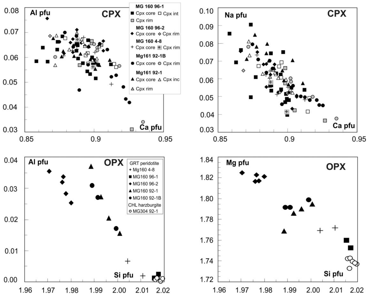
Fig. 8. Major element compositions of clinopyroxene and orthopyroxene from the Gagnone peridotites.
