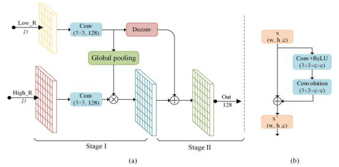
Fig. 4. The details of global context attention module and boundary refinement block are illustrated in (a) and (b), respectively.
