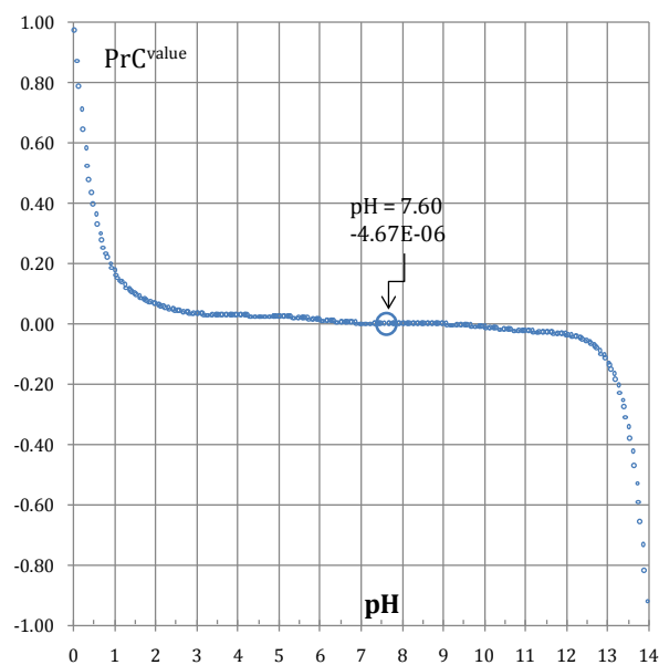
Figure 14. Plot PrC value → pH for the 0.00684 M H 4 EDTA + 0.020 M Na 4 EDTA mixture of Example 6.
