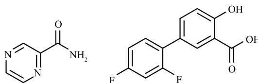
Pyrazinamide
