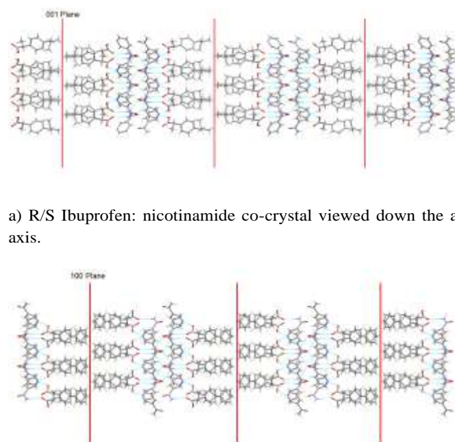
b) R/S flurbiprofen: nicotinamide co-crystal † viewed down the c-axis.
