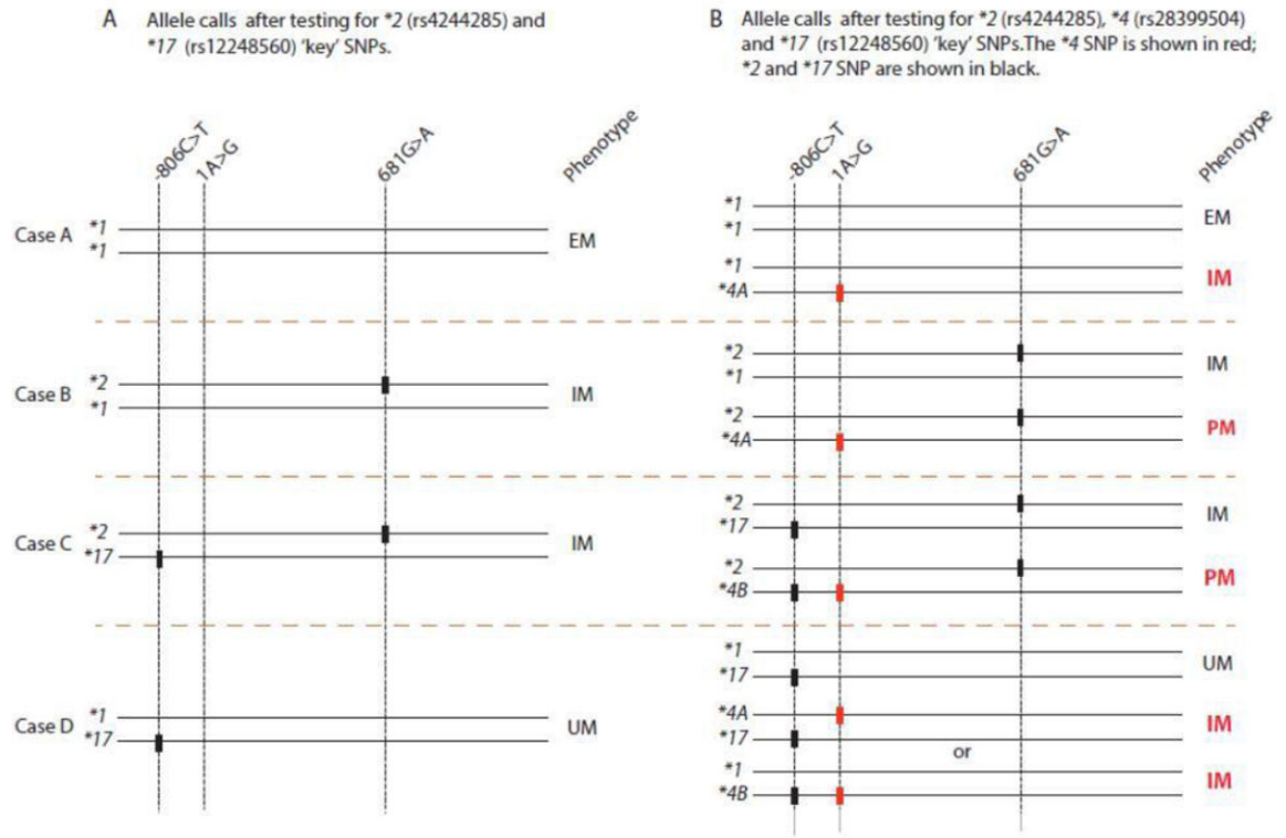
Figure 2. CYP2C19 *2, *4, and *17 alleles are used to illustrate how metabolizer phenotypes will be miscalled if CYP2C19 *2 and *17 but not CYP2C19 *4, are tested. Four possible scenarios are shown (Cases A-D). Panel A shows the phenotypes based on testing the key SNVs for CYP2C19 *2 and *17. Panel B shows the phenotypes based on testing the key variants for CYP2C19 *2, *4 and *17. Phenotypes shown in red in Panel B would have been miscalled if rs28399504 is present in the sample, but not included in the assay. These alleles are used as example, demonstrating that all alleles affecting CYP2C19 functionality should be interrogated in order to accurately call phenotypes. (PM = poor metabolizer; IM = intermediate metabolizer; EM = extensive metabolizer; UM = ultrarapid metabolizer)
