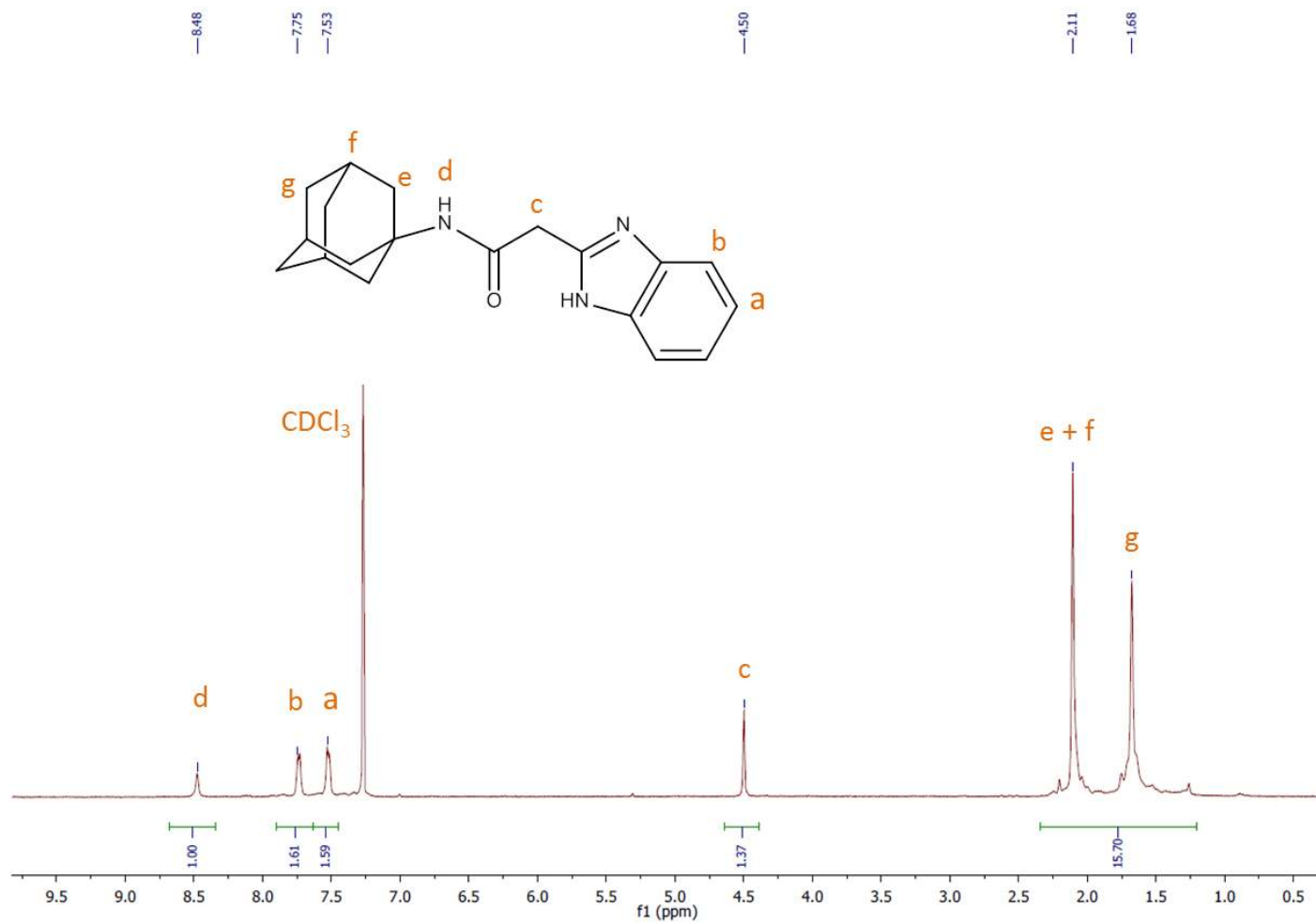
Figure 3.10. 1 H-NMR analysis of DML-4.
