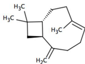
Figure 1.8. Chemical structure of \beta -caryophyllene.
