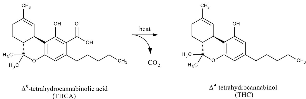
Figure 1.7. De-carboxylation of Δ 9 -tetrahydrocannabinolic acid (THCA) to Δ 9 -tetrahydrocannabinol (THC).
