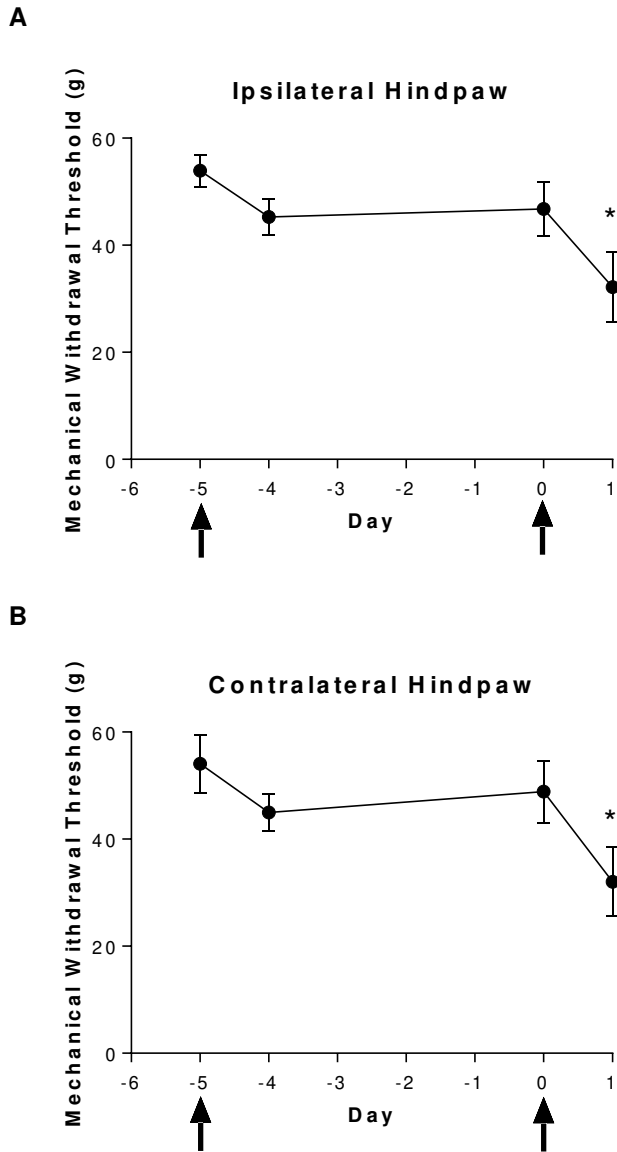
Figure 2.2. Pooled ipsilateral (A) and contralateral (B) hindpaw withdrawal thresholds from AS animals classified as bilateral hyperalgesia responders (n = 5). Arrows indicate days of acidic saline injections. Mechanical withdrawal thresholds were assessed thirty min prior to injection on injection days. Data points represent mean ± SD. * = P < 0.05 vs. all other experimental days.
