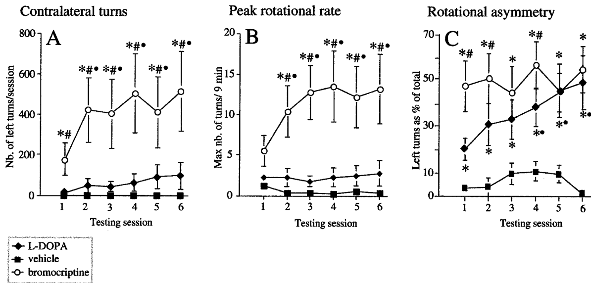
FIG. 5. Rotometry measurements during a 3-week course of treatment with L-DOPA (6 mg/kg/day combined with benserazide, 15 mg/kg; n = 14 ), bromocriptine (3.5 mg/kg/day; n = 14 ) or vehicle ( n = 8 ). (A) Total numbers of turns in the direction contralateral to the lesion; (B) peak rotational rates; (C) rotational asymmetries (i.e. percentages of contralateral turns in each recording session). P < 0.05 vs: *vehicle; #L-DOPA; ●testing session 1 in the same group.
