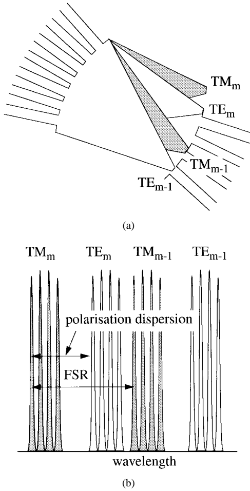
Fig. 6. Schematic diagram of the different diffraction orders at the receiver side for both states of polarization: Polarization dispersion.
