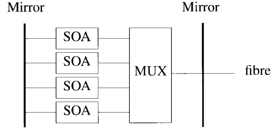
Fig. 12. Integrated multiwavelength laser.
