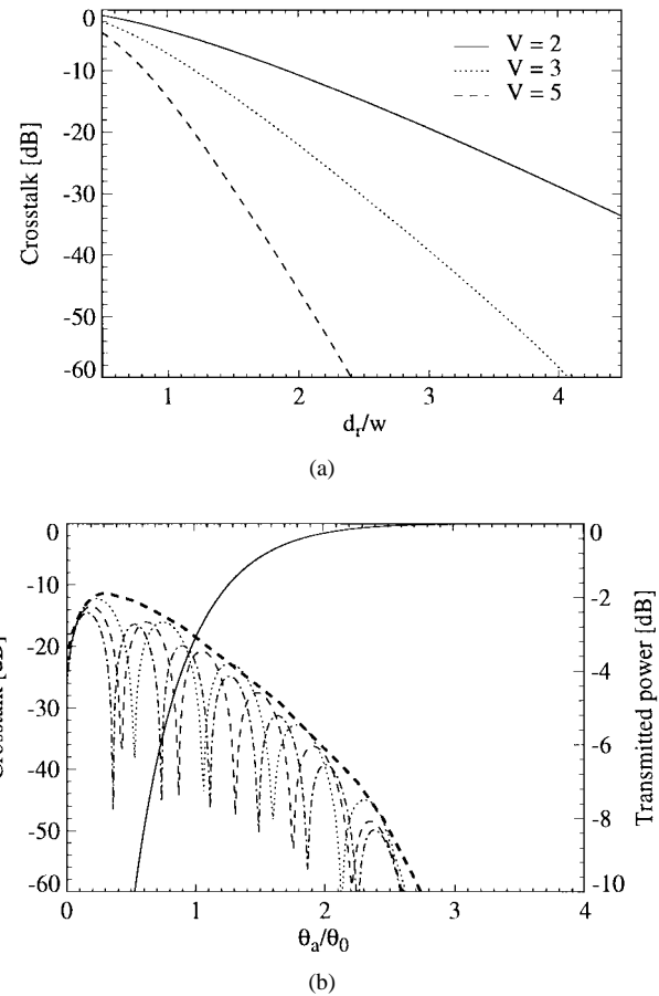
Fig. 3. (a) Crosstalk resulting from the coupling between two adjacent receiver channels for different values of the lateral V -parameter of the receiver waveguides. (b) Transmitted power (solid line) and crosstalk as a function of the relative array aperture \theta_a/\theta_0 , for different values of the relative receiver spacing d_r/w ( d_r/w = 2.5, 3.0, 3.5 ). The values shown are calculated for input and output waveguides with V = 3 . The bold line indicates the envelope of the crosstalk curves (maximum crosstalk level).
