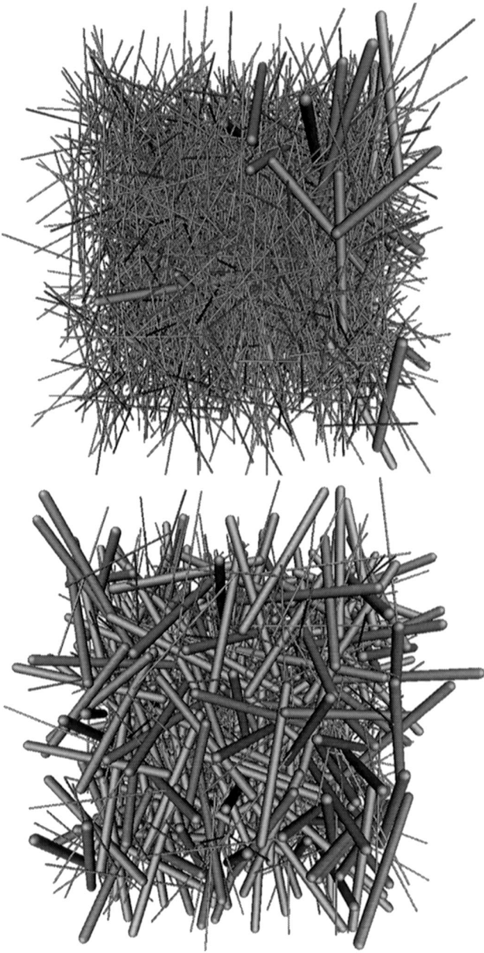
Fig. 5. Snapshots of two coexisting isotropic phases of a binary mixture of hard spherocylinders characterized by length-to-diameter ratios L/D_1 = 150 and L/D_2 = 15 , and hence by a diameter ratio d = D_2/D_1 = 10 . The compositions are x = 0.069 (upper), and x = 0.411 (lower).
