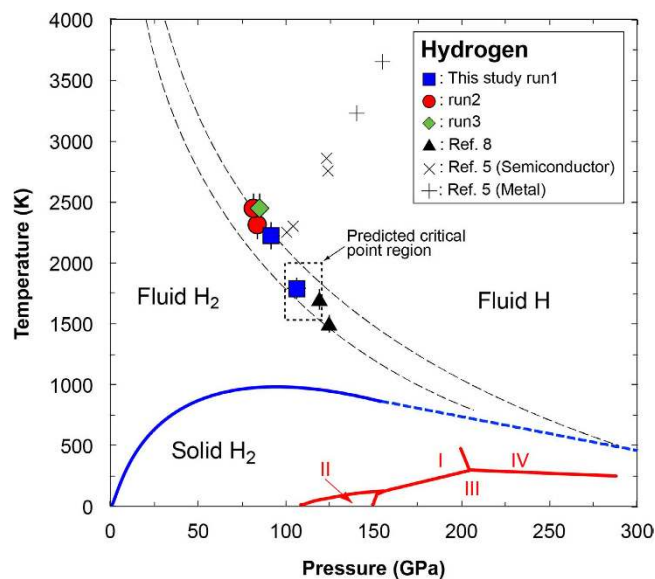
Figure 4. Phase diagram of dense hydrogen. For the plasma phase transition boundary, we show a range of curves resulting from reported theoretical calculations 10–13,15 by black broken lines. The predicted position of the critical point is indicated by dotted box 13 . Melting curve and phase boundaries of solid hydrogen are taken from the literature 8 . Cross and plus symbols represent P - T conditions at which electrical conductivities were measured under shock compression 5 .
