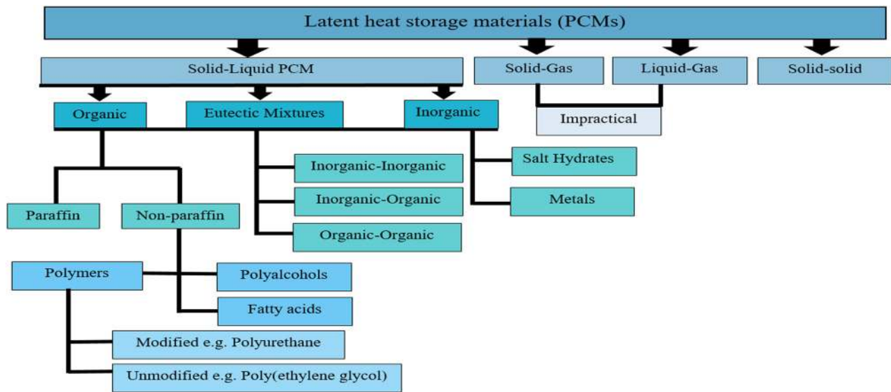
Figure 1: Classification of PCMs.
