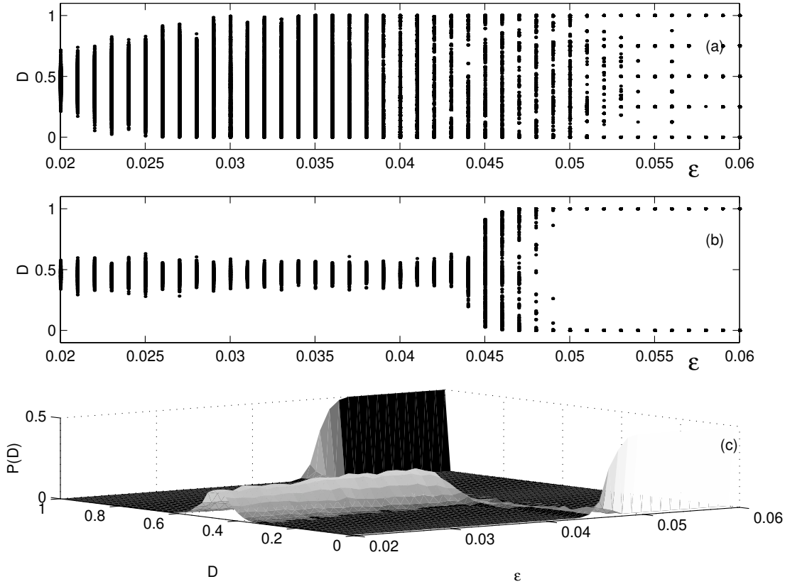
Fig. 1. (a) Normalized phase distances D versus \varepsilon for system (2) obtained from random initial conditions. A slow diffusion process in the phase distances leads eventually to the formation of a phase clustered state. (b) Same for system (1). Notice the sharp transition to a phase clustered state occurring now at \varepsilon \simeq 0.046 . (c) Three-dimensional graph reporting the probability distribution P(D) of the phase distances as a function of \varepsilon for system (1).
