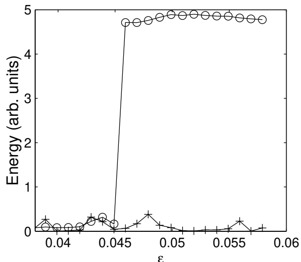
Fig. 3. Mean energy (see text for definition) of the lattice i = 50 in both coupled (open circles) and uncoupled (crosses) cases. The cooperative effects of the coupling can be fully appreciated in the sharp rise of the mean field energy for system (1).
