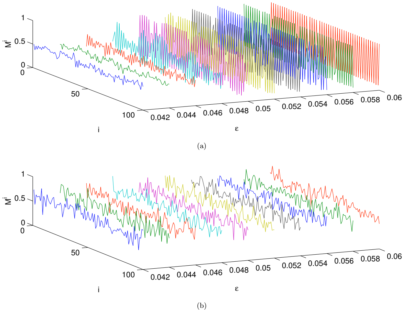
Fig. 2. Three-dimensional plots of the mean fields \mathcal{M}^i (at a fixed time) as functions of i and \epsilon for (a) system (1) and (b) system (2). In (a) a spatial period 2 appears when crossing \epsilon \simeq 0.046 , and in (b) one cannot appreciate qualitative changes in the behavior of the \mathcal{M} 's values for the studied range of coupling strength. In both cases the color code has been chosen only to make more understandable the appearance of the spatial structure.
