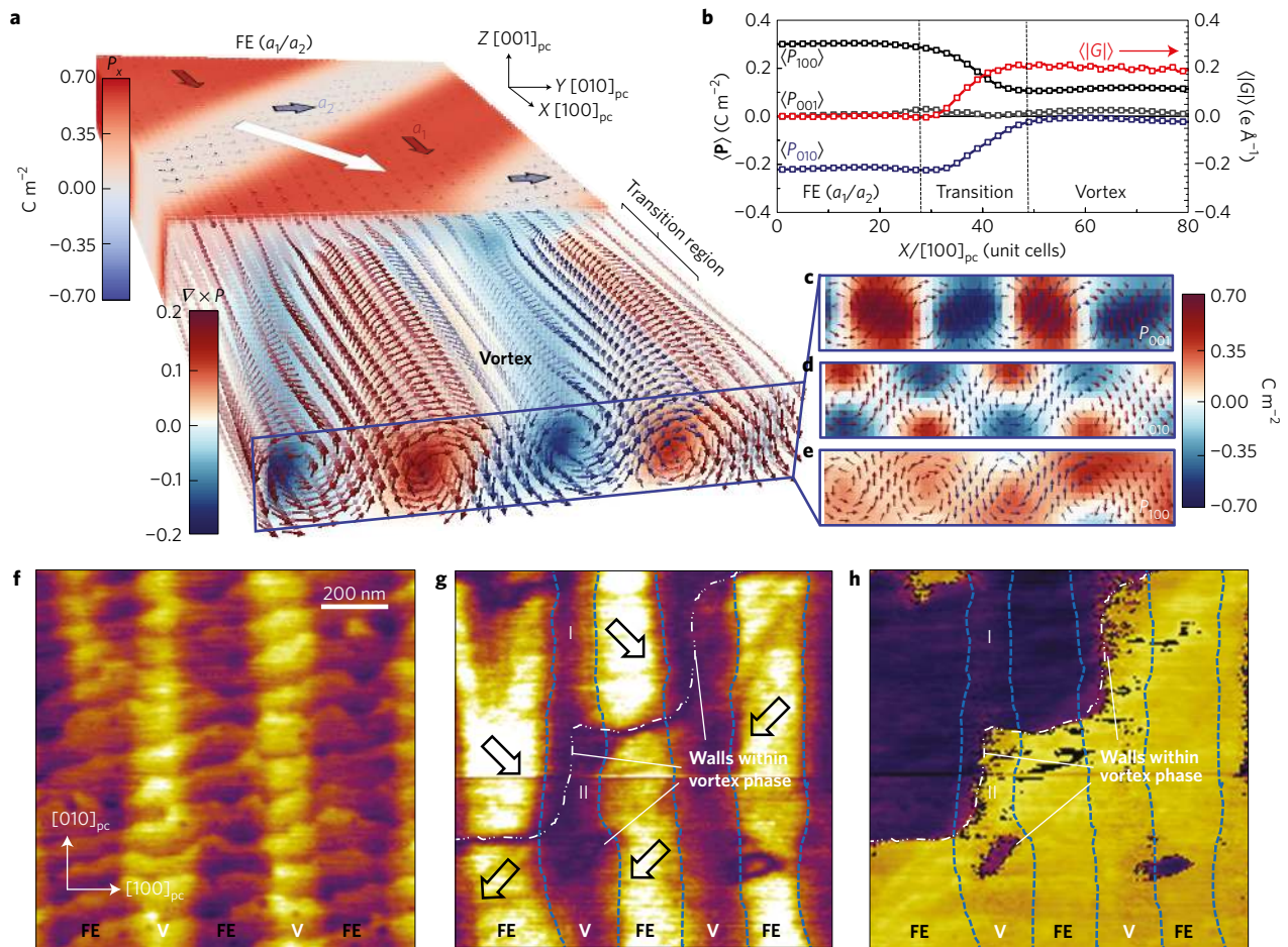
Figure 3 | Exploring the phase boundary between a_1/a_2 and vortex phases. a , A zoom-in of the phase-field calculation focusing on a single PbTiO 3 layer near the phase boundary and revealing that the ferroelectric a_1/a_2 superdomain (labelled FE( a_1/a_2 ), colour scale showing polarization component along [100] pc or the X-direction) smoothly transitions to the vortex phase (labelled Vortex, colour scale corresponding to magnitude of \nabla \times P ) comprising of alternating clockwise and anticlockwise polarization vortices. b , Plot showing the spatially averaged ferroelectric polarization components ( \langle P_{001} \rangle , \langle P_{010} \rangle and \langle P_{100} \rangle ) and the averaged magnitude of the axial electrical toroidal moment ( \langle |G| \rangle ) as one traverses across the phase boundary along [100] from the ferroelectric to the vortex phase. c–e are colour-maps showing the spatial distribution of the (c) P_{001} , (d) P_{010} and (e) P_{100} components for a cross-section (blue box, a ) of the vortex phase and highlight the coexistence of toroidization and an axial component ( P_{100} \approx 0.1 \text{ C m}^{-2} ) of polarization, the direction of which is related to polarization in the adjacent a_1/a_2 phase. f–h , Lateral piezoresponse force studies showing (f) topography, (g) lateral amplitude, and (h) lateral phase revealing the nanoscale distribution of a_1/a_2 and vortex phases, and highlighting the presence of domain-wall-like features within the vortex phase that are indicative of axial polarization components.
