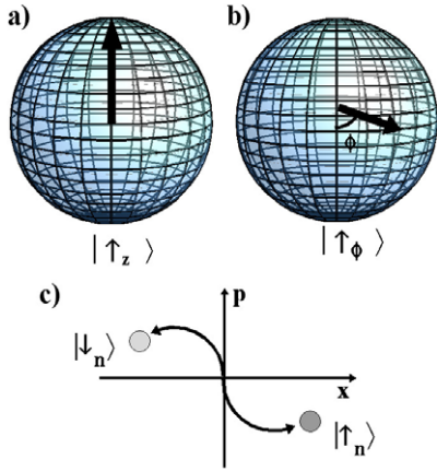
Figure 5. Representation of the eigenstate of (a) \sigma \cdot z and (b) \sigma \cdot \phi on the Bloch sphere corresponding to the eigenvalue +1. A spin-dependent force creates two separate coherent states in phase space corresponding to the eigenstates of \sigma \cdot n , as represented in (c), thus entangling the internal spin with the external motion of the ion.
