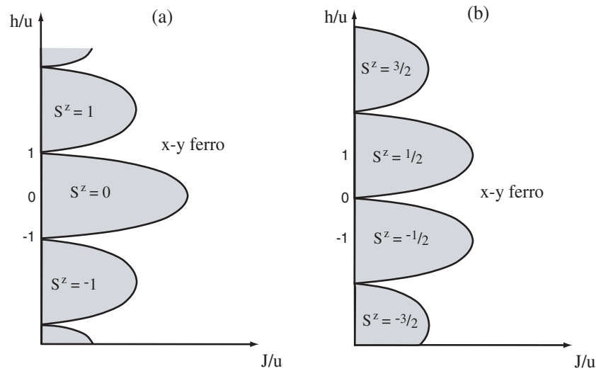
Figure 2. Phase diagram of the Mott state with 0 < V_{a,b} - U \ll U and (a) even and (b) odd total filling. The filled lobes mark Mott states with fixed S^z = (n_a - n_b)/2 . Outside of these lobes the system is also in a Mott state but with x - y ferromagnetic spin order.
