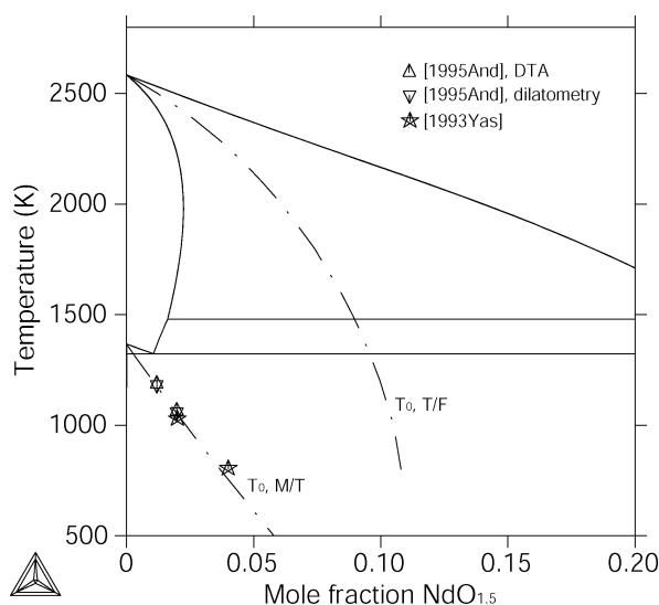
Fig. 3 Calculated \text{ZrO}_2\text{-NdO}_{1.5} partial phase diagram, and T_0 lines for monoclinic + tetragonal and tetragonal + fluorite equilibria together with experimental data.
