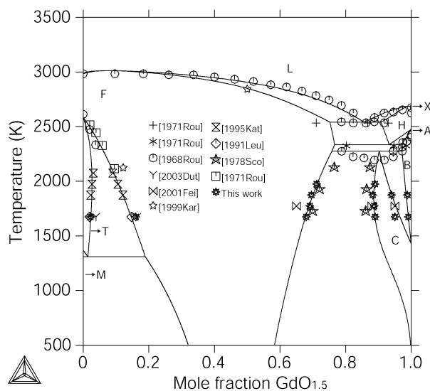
Fig. 6 Calculated ZrO 2 -GdO 1.5 phase diagram without the pyrochlore phase compared with experimental data.
