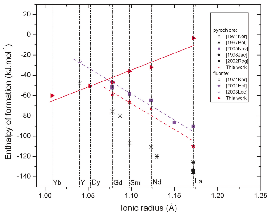
Fig. 19 Experimental and calculated enthalpies of formation of pyrochlore and fluorite (per four moles of cations, reference state: the monoclinic ZrO_2 and the stable structure of REO_{1.5} at room temperature, for the composition at 50 mol % REO_{1.5} ).
