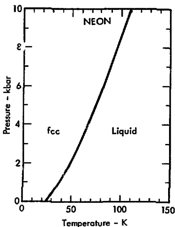
Fig. 14. The phase diagram of neon.
