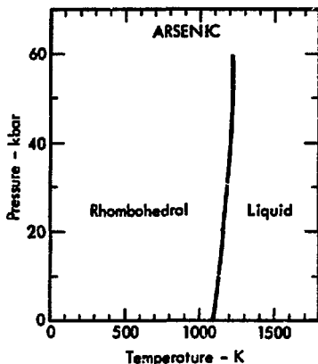
Fig. 35. The phase diagram of arsenic.
