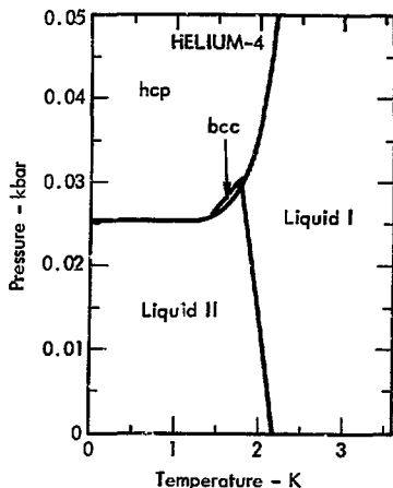
Fig. 6. The phase diagram of helium - 4.
