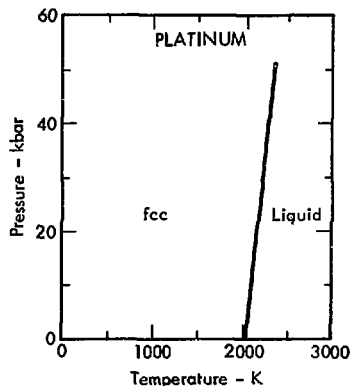
Fig. 70. The phase diagram of platinum.
