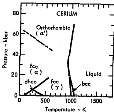
Fig. 55. The phase diagram of cerium.
