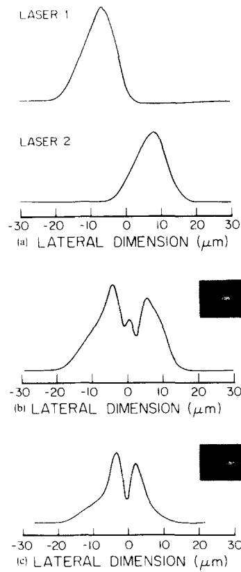
FIG. 4. Near-field distributions (in the junction plane) obtained under the same operation conditions as in Fig. 3. (a) The individual laser near fields. (b) Near field of the phase-locked lasers operating in the even (+ +) supermode. (c) Near field of the phase-locked lasers operating in the odd (+ -) supermode. The inserts show the near field photographs.
