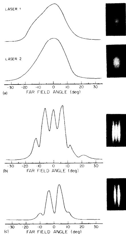
FIG. 3. Far-field photographs and far-field distributions (in the junction plane). (a) Far fields of each laser operating by itself at I_1 or I_2 = 350 mA ( J_n = 300 mA). (b) Far field for I_1 = 180 mA, I_2 = 160 mA. The two lasers are locked in phase (even supermode). (c) Far field for I_1 = 150 mA, I_2 = 180 mA. The lasers are locked \pi rad out of phase (odd supermode).
