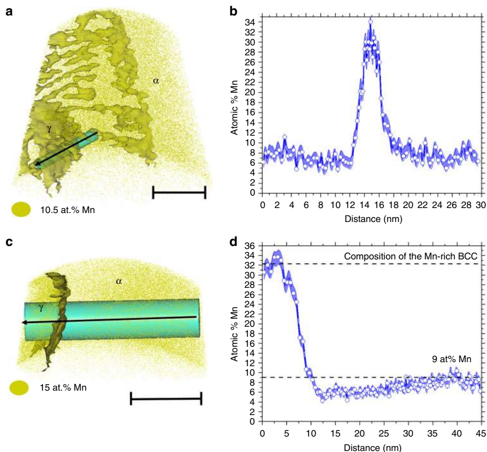
Fig. 7 Composition of the austenite after 6 h and 2 weeks at 450 °C. a, b Fe-9 atomic % Mn solid solution, 50% cold-rolled, and annealed at 450 °C for 6 h: a APT reconstruction showing an austenite nucleus sited on an LAGB or a triple junction of LAGB. b 1D compositional profile along the cylinder showed in a . c, d Fe-9 atomic % Mn solid solution, 50% cold-rolled, and annealed at 450 °C for 2 weeks: c APT reconstruction showing an austenite nucleus in initial stage of growth. d 1D compositional profile along the cylinder showed in c . \alpha represents the BCC-ferrite phase and \gamma represents the FCC-austenite phase. The points in b, d are the experimental values, which are connected by blue lines. The blue shading represents the statistical error associated with the calculation of the composition
