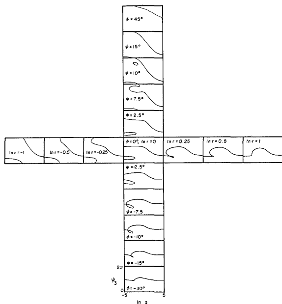
Fig. 2. Numerical curves of \psi_3 versus \ln q for various \ln r and \phi . |\gamma l| was chosen to be 6. For each of the curves, the range of \psi_3 is from 0 to 2\pi and from -5 to 5 for \ln q .
