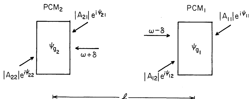
Fig. 3. Schematic diagram of a double phase-conjugate resonator.
