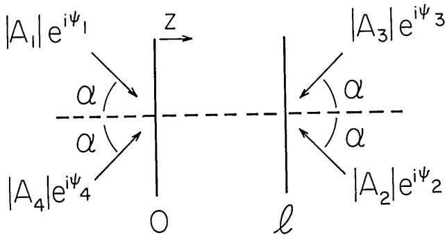
Fig. 1. Schematic diagram of nonlinear four-wave mixing in a nonlinear medium. A_1 and A_2 are the pumping beams, A_3 is the phase-conjugate output, and A_4 is the probe beam.
