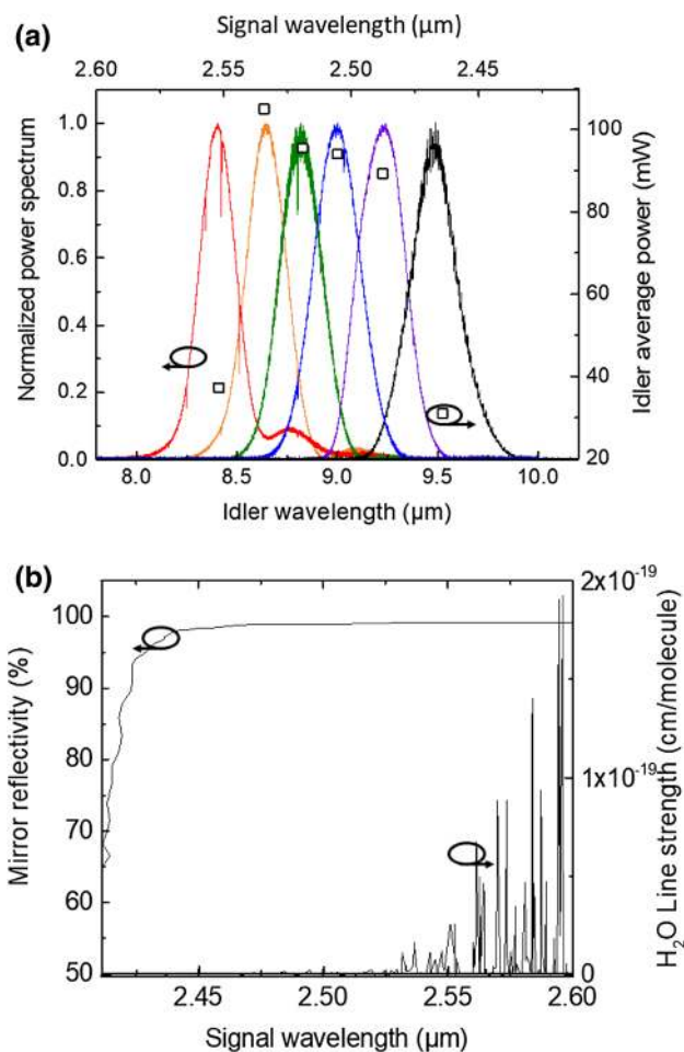
Fig. 3 OPO wavelength tuning. a Idler spectrum and corresponding idler average power. b Reflectivity of input mirror M1 (left) and the line strength of water rovibrational features (right) as a function of signal wavelength
