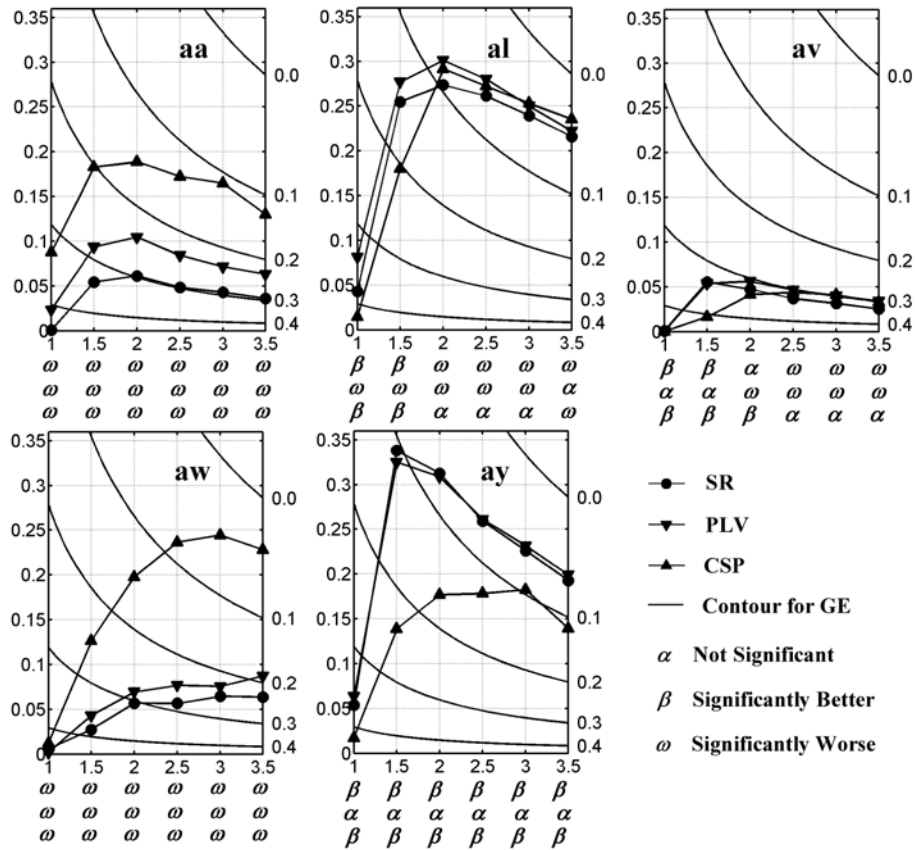
Figure 3: Information transfer rates (ITR) for synchrony rate (SR), PLV and CSP method. Horizontal axis is time T (in seconds). Vertical axis on the left measures information transfer rate (in bit/second) and that on the right shows the generalization error (GE) in decimals. The three lines of Greek characters under each subplot code the results of statistical comparisons (Student's t-test, significance level 0.01) of different methods. Line 1 is the comparison between SR and CSP methods; Line 2 is between SR and PLV method; and Line 3 between PLV and CSP method.
