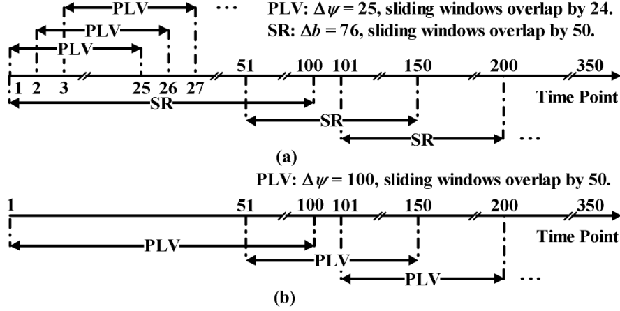
Figure 1: Overall scheme of window division for (a) the synchrony rate (SR) method and (b) the phase locking value (PLV) method. \Delta\psi for the SR method covers the length of a micro-window, while that for the PLV method corresponds to the length of a sliding window. \Delta_b is equal to 100 - \Delta\psi + 1 . (Note: time axis is NOT uniformly scaled.)
